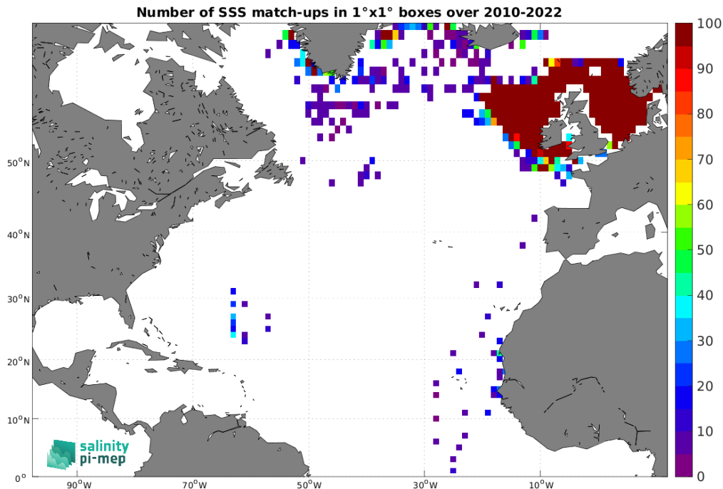
Figure 5: Number of SSS match-ups between ICES SSS and the SMOS SSS L3 v332 - 9 Days (CATDS-CPDC) SSS product for the North Atlantic Ocean Pi-MEP region over 1^\circ \times 1^\circ boxes and for the full satellite product period.
