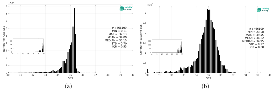
Figure 3: Histograms of SSS from ICES (a) and SMOS SSS L3 v332 - 9 Days (CATDS-CPDC) (b) considering all match-up pairs per bins of 0.1 over the North Atlantic Ocean Pi-MEP region and for the full satellite product period.
