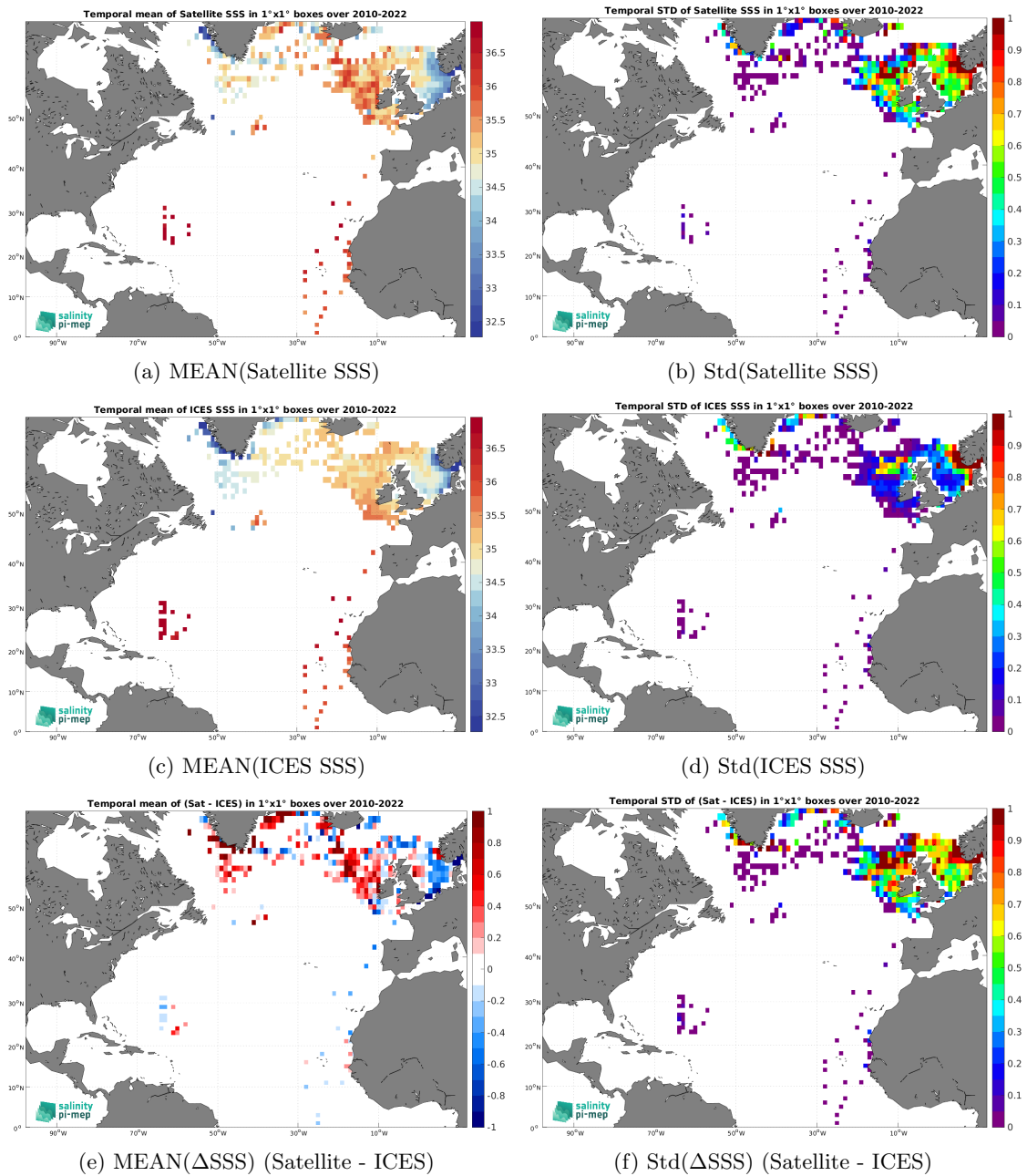
Figure 7: Temporal mean (left) and Std (right) of SSS from SMOS SSS L3 v332 - 9 Days (CATDS-CPDC) (top), ICES (middle), and of \Delta SSS (Satellite - ICES). Only match-up pairs are used to generate these maps.
