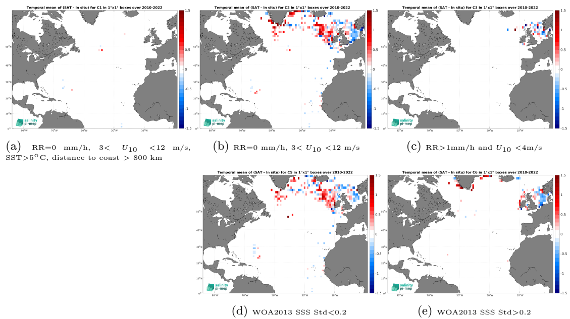
Figure 14: Temporal mean gridded over spatial boxes of size 1^\circ \times 1^\circ of \Delta SSS (SMOS SSS L3 v332 - 9 Days (CATDS-CPDC) - ICES) for 5 different subdatasets corresponding to:RR=0 mm/h, 3 < U_{10} < 12 m/s, SST > 5°C, distance to coast > 800 km (a), RR=0 mm/h, 3 < U_{10} < 12 m/s (b), RR > 1mm/h and U_{10} < 4 m/s (c), WOA2013 SSS Std < 0.2 (d), WOA2013 SSS Std > 0.2 (e).
