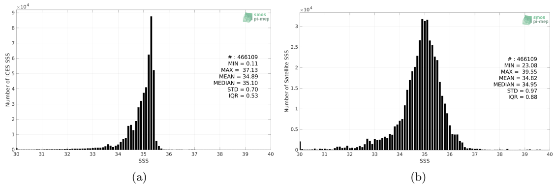
Figure 2: Histograms of SSS from ICES (a) and SMOS SSS L3 v332 - 9 Days (CATDS-CPDC) (b) considering all match-up pairs per bins of 0.1 over the North Atlantic Ocean Pi-MEP region and for the full satellite product period.
