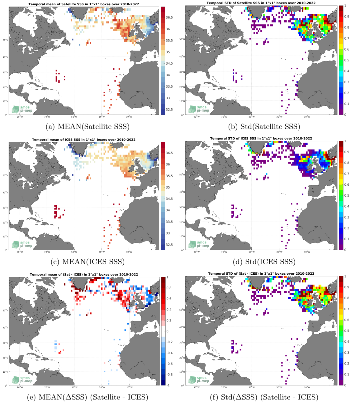
Figure 6: Temporal mean (left) and Std (right) of SSS from SMOS SSS L3 v332 - 9 Days (CATDS-CPDC) (top), ICES (middle), and of \Delta SSS (Satellite - ICES). Only match-up pairs are used to generate these maps.
