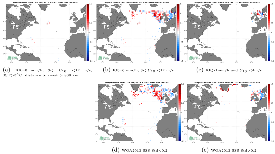
Figure 12: Temporal mean gridded over spatial boxes of size 1^\circ \times 1^\circ of \Delta\text{SSS} (SMOS SSS L3 v332 - 9 Days (CATDS-CPDC) - ICES) for 5 different subdatasets corresponding to:RR=0 mm/h, 3 < U_{10} < 12 m/s, SST >5^\circ\text{C} , distance to coast > 800 km (a), RR=0 mm/h, 3 < U_{10} < 12 m/s (b), RR >1 mm/h and U_{10} < 4 m/s (c), WOA2013 SSS Std <0.2 (d), WOA2013 SSS Std >0.2 (e).
