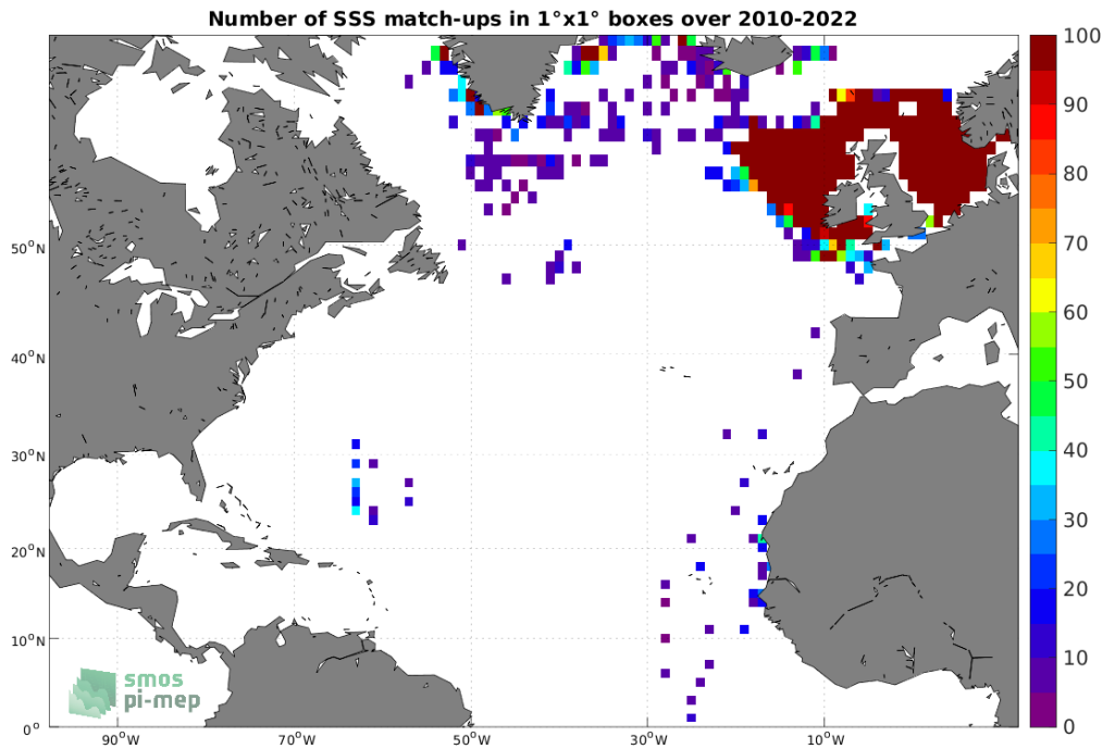
Figure 4: Number of SSS match-ups between ICES SSS and the SMOS SSS L3 v332 - 9 Days (CATDS-CPDC) SSS product for the North Atlantic Ocean Pi-MEP region over 1^\circ \times 1^\circ boxes and for the full satellite product period.
