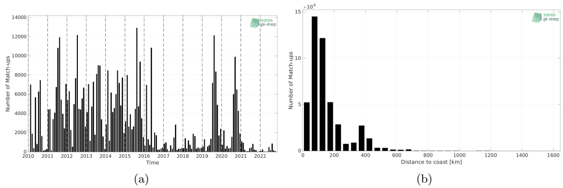
Figure 1: Number of match-ups between ICES and SMOS SSS L3 v332 - 9 Days (CATDS-CPDC) SSS as a function of time (a) and as function of the distance to coast (b) over the North Atlantic Ocean Pi-MEP region and for the full satellite product period.
