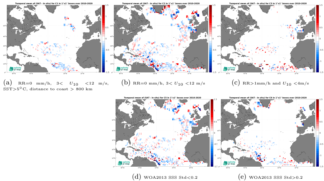
Figure 13: Temporal mean gridded over spatial boxes of size 1^\circ \times 1^\circ of \Delta\text{SSS} (SMOS SSS L3 v332 - 9 Days (CATDS-CPDC) - Surface drifters) for 5 different subdatasets corresponding to:RR=0 mm/h, 3 < U_{10} < 12 m/s, SST >5^\circ\text{C} , distance to coast > 800 km (a), RR=0 mm/h, 3 < U_{10} < 12 m/s (b), RR >1 mm/h and U_{10} < 4 m/s (c), WOA2013 SSS Std <0.2 (d), WOA2013 SSS Std >0.2 (e).
