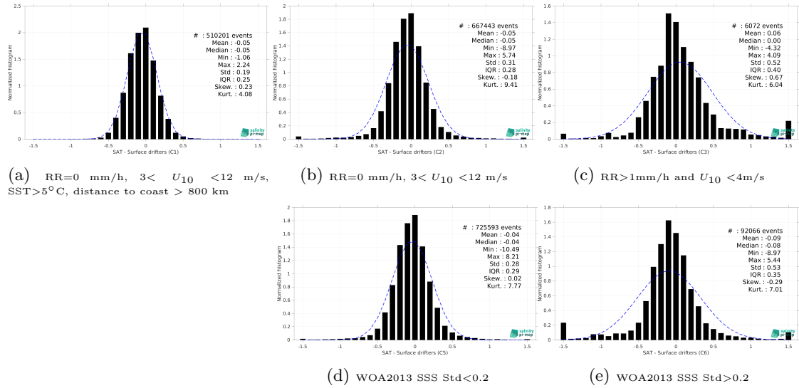
Figure 12: Normalized histogram of \Delta\text{SSS} (SMOS SSS L3 v332 - 9 Days (CATDS-CPDC) - Surface drifters) for 5 different subdatasets corresponding to: RR=0 mm/h, 3 < U_{10} < 12 m/s, SST>5°C, distance to coast > 800 km (a), RR=0 mm/h, 3 < U_{10} < 12 m/s (b), RR>1mm/h and U_{10} < 4 m/s (c), WOA2013 SSS Std<0.2 (d), WOA2013 SSS Std>0.2 (e).
