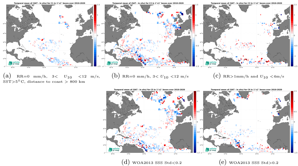
Figure 11: Temporal mean gridded over spatial boxes of size 1^\circ \times 1^\circ of \Delta\text{SSS} (SMOS SSS L3 v332 - 9 Days (CATDS-CPDC) - Surface drifters) for 5 different subdatasets corresponding to:RR=0 mm/h, 3 < U_{10} < 12 m/s, SST >5^\circ\text{C} , distance to coast > 800 km (a), RR=0 mm/h, 3 < U_{10} < 12 m/s (b), RR >1 mm/h and U_{10} < 4 m/s (c), WOA2013 SSS Std <0.2 (d), WOA2013 SSS Std >0.2 (e).
