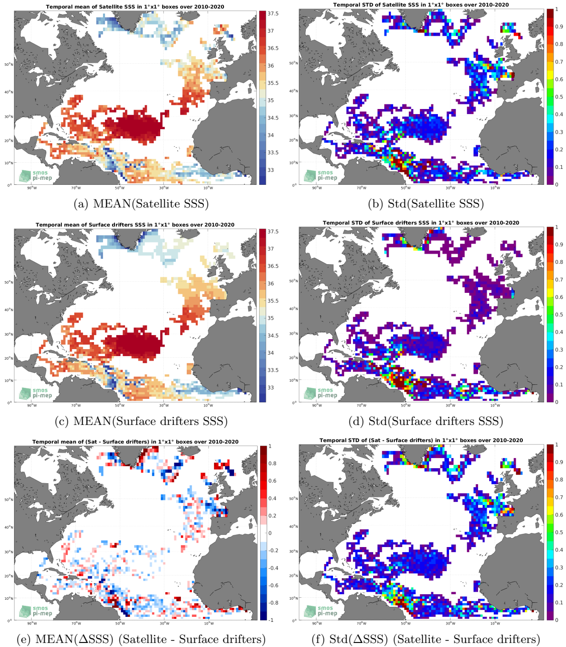
Figure 5: Temporal mean (left) and Std (right) of SSS from SMOS SSS L3 v332 - 9 Days (CATDS-CPDC) (top), Surface drifters (middle), and of \Delta SSS (Satellite - Surface drifters). Only match-up pairs are used to generate these maps.
