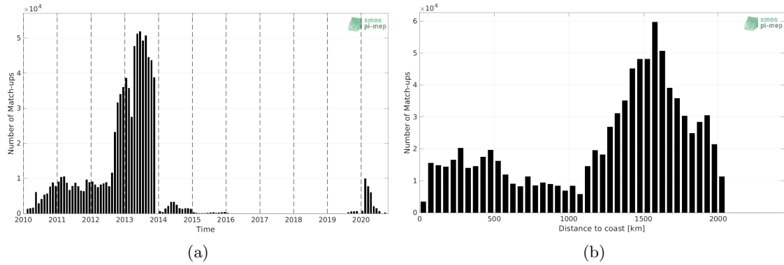
Figure 1: Number of match-ups between Surface drifters and SMOS SSS L3 v332 - 9 Days (CATDS-CPDC) SSS as a function of time (a) and as function of the distance to coast (b) over the North Atlantic Ocean Pi-MEP region and for the full satellite product period.
