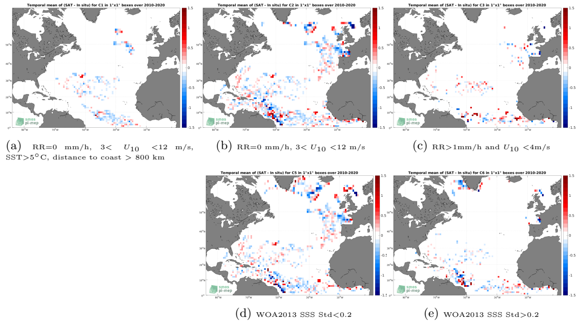
Figure 11: Temporal mean gridded over spatial boxes of size 1^\circ \times 1^\circ of \Delta SSS (SMOS SSS L3 v332 - 9 Days (CATDS-CPDC) - Surface drifters) for 5 different subdatasets corresponding to:RR=0 mm/h, 3 < U_{10} < 12 m/s, SST >5^\circ C, distance to coast > 800 km (a), RR=0 mm/h, 3 < U_{10} < 12 m/s (b), RR >1 mm/h and U_{10} < 4 m/s (c), WOA2013 SSS Std <0.2 (d), WOA2013 SSS Std >0.2 (e).
