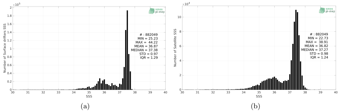
Figure 2: Histograms of SSS from Surface drifters (a) and SMOS SSS L3 v332 - 9 Days (CATDS-CPDC) (b) considering all match-up pairs per bins of 0.1 over the North Atlantic Ocean Pi-MEP region and for the full satellite product period.
