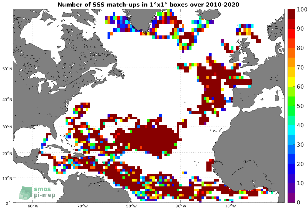
Figure 3: Number of SSS match-ups between Surface drifters SSS and the SMOS SSS L3 v332 - 9 Days (CATDS-CPDC) SSS product for the North Atlantic Ocean Pi-MEP region over 1^\circ \times 1^\circ boxes and for the full satellite product period.
