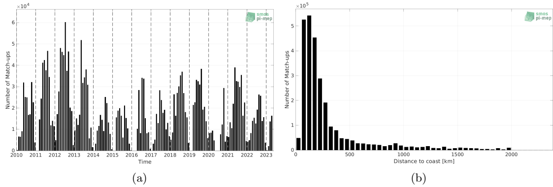
Figure 1: Number of match-ups between TSG (SAMOS) and SMOS SSS L2Q v331 - 0.25 Deg (CATDS-CPDC) SSS as a function of time (a) and as function of the distance to coast (b) over the North Atlantic Ocean Pi-MEP region and for the full satellite product period.
