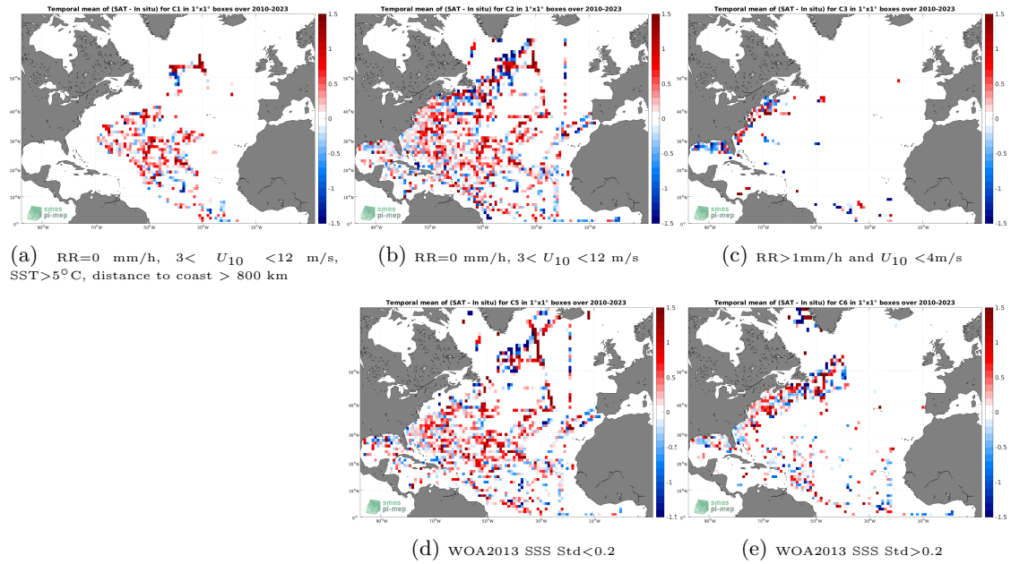
Figure 12: Temporal mean gridded over spatial boxes of size 1^\circ \times 1^\circ of \Delta\text{SSS} (SMOS SSS L2Q v331 - 0.25 Deg (CATDS-CPDC) - TSG (SAMOS)) for 5 different subdatasets corresponding to:RR=0 mm/h, 3 < U_{10} < 12 m/s, SST >5^\circ\text{C} , distance to coast > 800 km (a), RR=0 mm/h, 3 < U_{10} < 12 m/s (b), RR >1 mm/h and U_{10} < 4 m/s (c), WOA2013 SSS Std <0.2 (d), WOA2013 SSS Std >0.2 (e).
