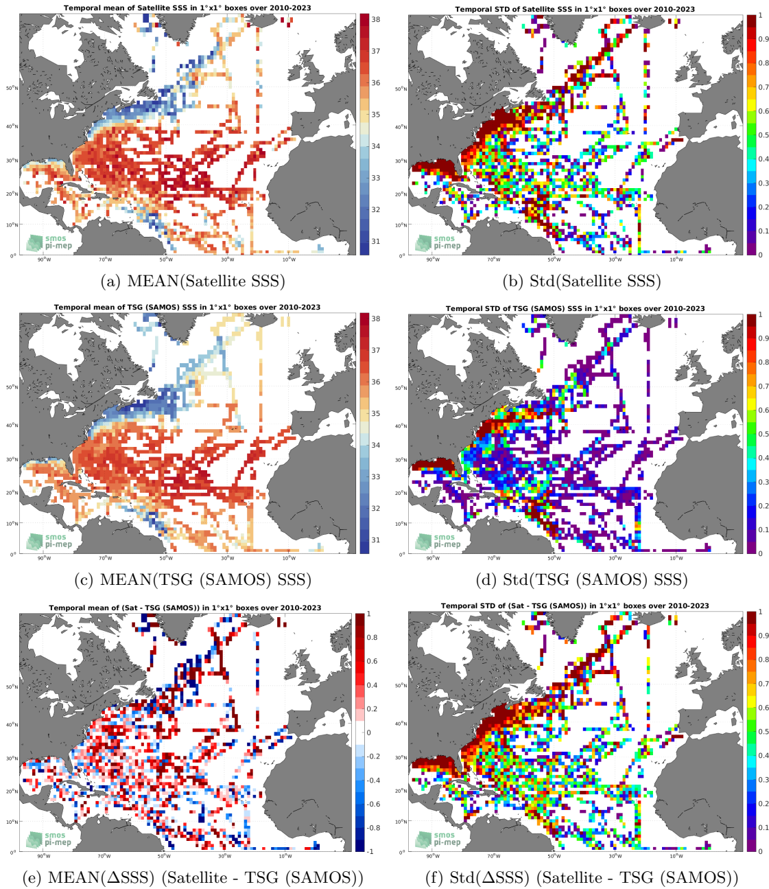
Figure 6: Temporal mean (left) and Std (right) of SSS from SMOS SSS L2Q v331 - 0.25 Deg (CATDS-CPDC) (top), TSG (SAMOS) (middle), and of \Delta SSS (Satellite - TSG (SAMOS)). Only match-up pairs are used to generate these maps.
