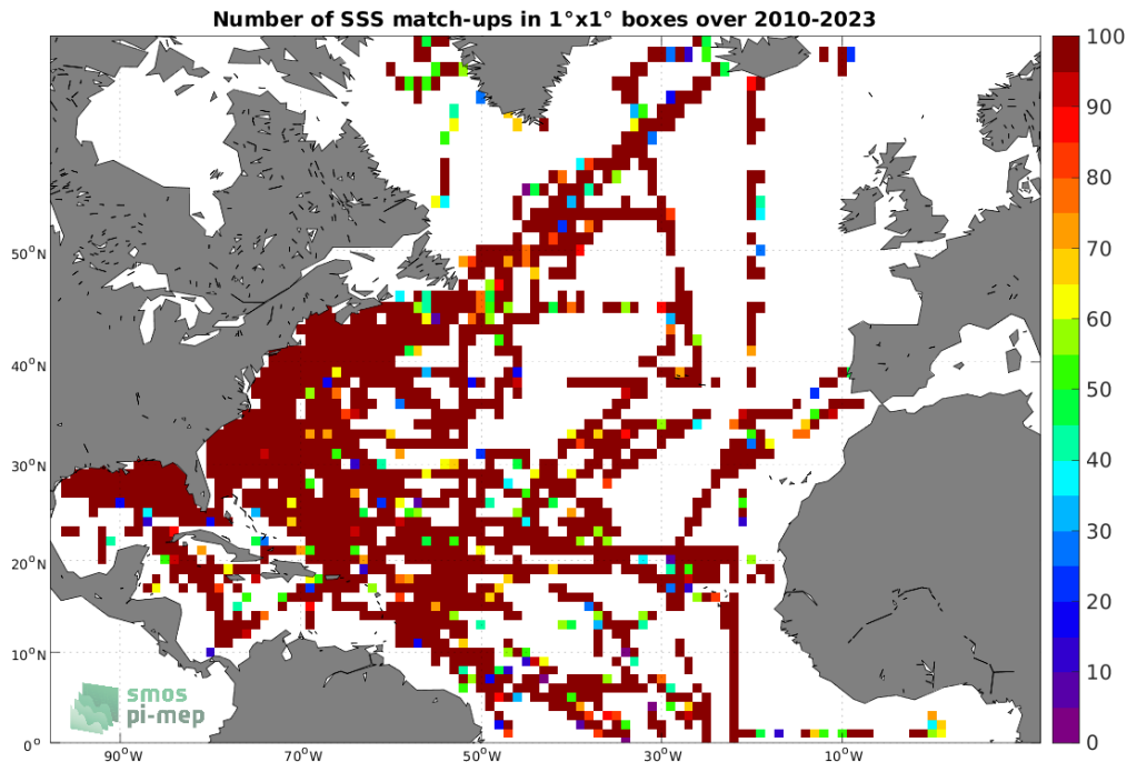
Figure 4: Number of SSS match-ups between TSG (SAMOS) SSS and the SMOS SSS L2Q v331 - 0.25 Deg (CATDS-CPDC) SSS product for the North Atlantic Ocean Pi-MEP region over 1^\circ \times 1^\circ boxes and for the full satellite product period.
