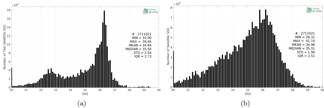
Figure 2: Histograms of SSS from TSG (SAMOS) (a) and SMOS SSS L2Q v331 - 0.25 Deg (CATDS-CPDC) (b) considering all match-up pairs per bins of 0.1 over the North Atlantic Ocean Pi-MEP region and for the full satellite product period.
