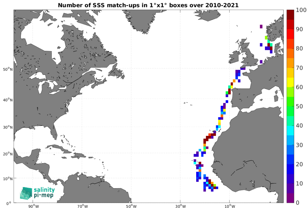
Figure 4: Number of SSS match-ups between TSG (Polarstern) SSS and the SMOS SSS L2Q v331 - 0.25 Deg (CATDS-CPDC) SSS product for the North Atlantic Ocean Pi-MEP region over 1^\circ \times 1^\circ boxes and for the full satellite product period.
