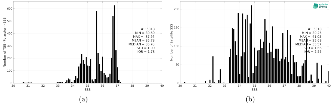
Figure 2: Histograms of SSS from TSG (Polarstern) (a) and SMOS SSS L2Q v331 - 0.25 Deg (CATDS-CPDC) (b) considering all match-up pairs per bins of 0.1 over the North Atlantic Ocean Pi-MEP region and for the full satellite product period.
