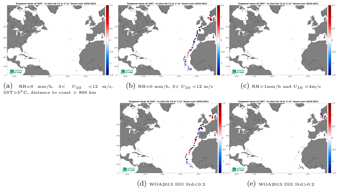
Figure 12: Temporal mean gridded over spatial boxes of size 1^\circ \times 1^\circ of \Delta\text{SSS} (SMOS SSS L2Q v331 - 0.25 Deg (CATDS-CPDC) - TSG (Polarstern)) for 5 different subdatasets corresponding to:RR=0 mm/h, 3 < U_{10} < 12 m/s, SST >5^\circ\text{C} , distance to coast > 800 km (a), RR=0 mm/h, 3 < U_{10} < 12 m/s (b), RR >1 mm/h and U_{10} < 4 m/s (c), WOA2013 SSS Std <0.2 (d), WOA2013 SSS Std >0.2 (e).
