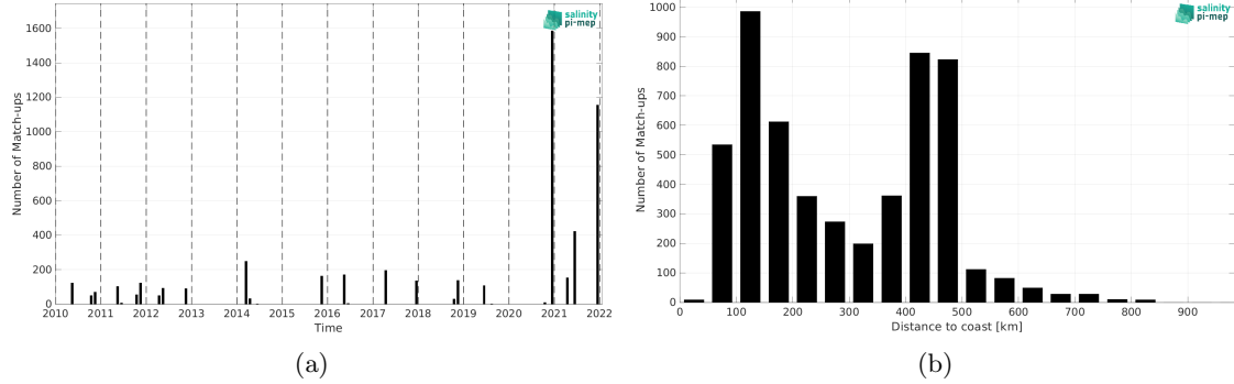
Figure 1: Number of match-ups between TSG (Polarstern) and SMOS SSS L2Q v331 - 0.25 Deg (CATDS-CPDC) SSS as a function of time (a) and as function of the distance to coast (b) over the North Atlantic Ocean Pi-MEP region and for the full satellite product period.
