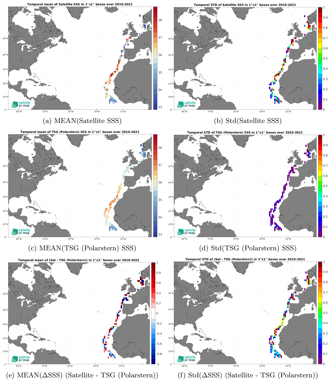
Figure 6: Temporal mean (left) and Std (right) of SSS from SMOS SSS L2Q v331 - 0.25 Deg (CATDS-CPDC) (top), TSG (Polarstern) (middle), and of \Delta SSS (Satellite - TSG (Polarstern)). Only match-up pairs are used to generate these maps.
