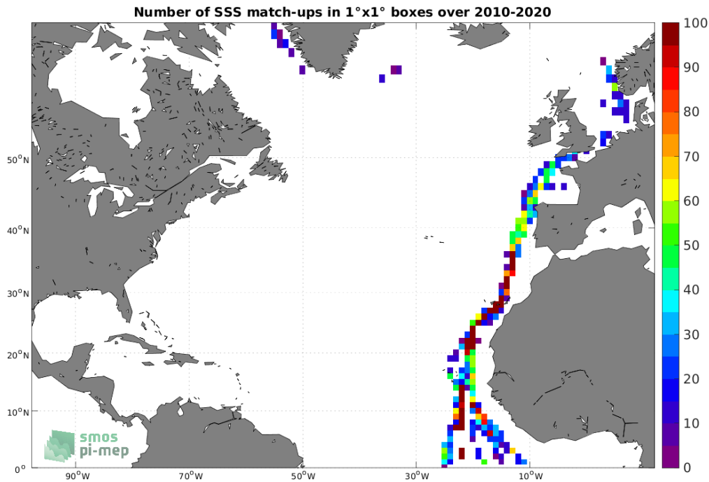
Figure 4: Number of SSS match-ups between TSG (Polarstern) SSS and the SMOS SSS L2Q v331 - 0.25 Deg (CATDS-CPDC) SSS product for the North Atlantic Ocean Pi-MEP region over 1°x1° boxes and for the full satellite product period.
