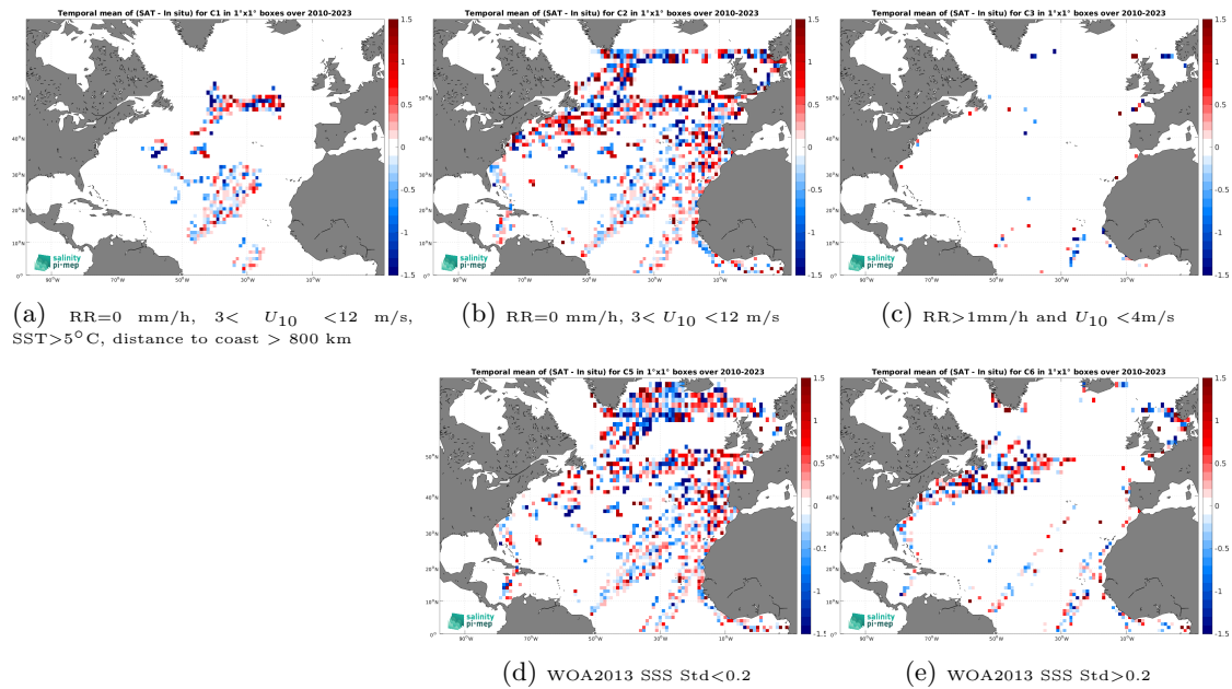
Figure 12: Temporal mean gridded over spatial boxes of size 1^\circ \times 1^\circ of \Delta\text{SSS} (SMOS SSS L2Q v331 - 0.25 Deg (CATDS-CPDC) - TSG (LEGOS-DM)) for 5 different subdatasets corresponding to:RR=0 mm/h, 3 < U_{10} < 12 m/s, SST >5^\circ\text{C} , distance to coast > 800 km (a), RR=0 mm/h, 3 < U_{10} < 12 m/s (b), RR >1 mm/h and U_{10} < 4 m/s (c), WOA2013 SSS Std <0.2 (d), WOA2013 SSS Std >0.2 (e).
