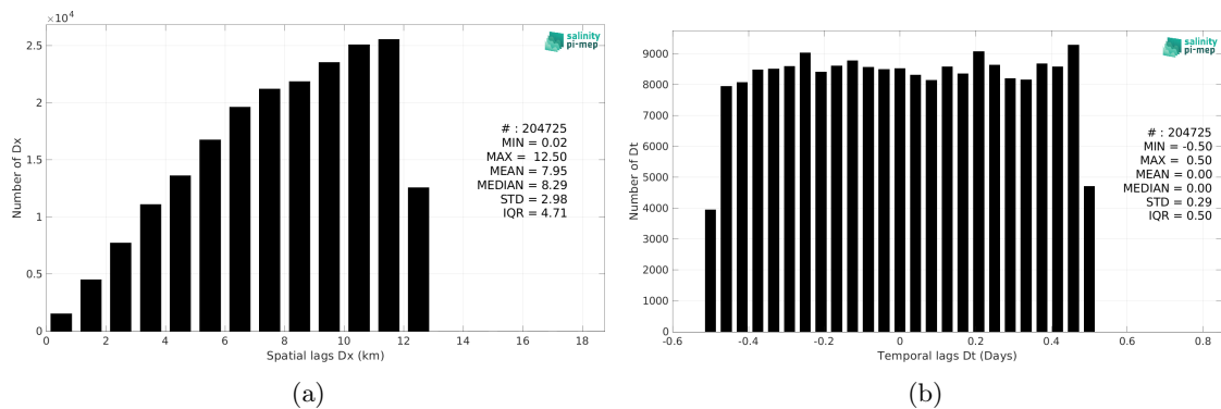
Figure 5: Histograms of the spatial (a) and temporal (b) lags between the location/time of the TSG (LEGOS-DM) measurement and the date of the corresponding SMOS SSS L2Q v331 - 0.25 Deg (CATDS-CPDC) SSS pixel.
