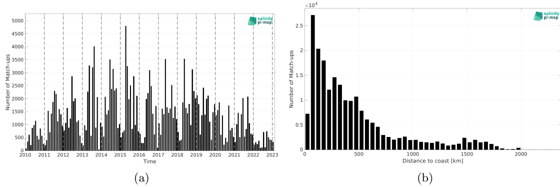
Figure 1: Number of match-ups between TSG (LEGOS-DM) and SMOS SSS L2Q v331 - 0.25 Deg (CATDS-CPDC) SSS as a function of time (a) and as function of the distance to coast (b) over the North Atlantic Ocean Pi-MEP region and for the full satellite product period.
