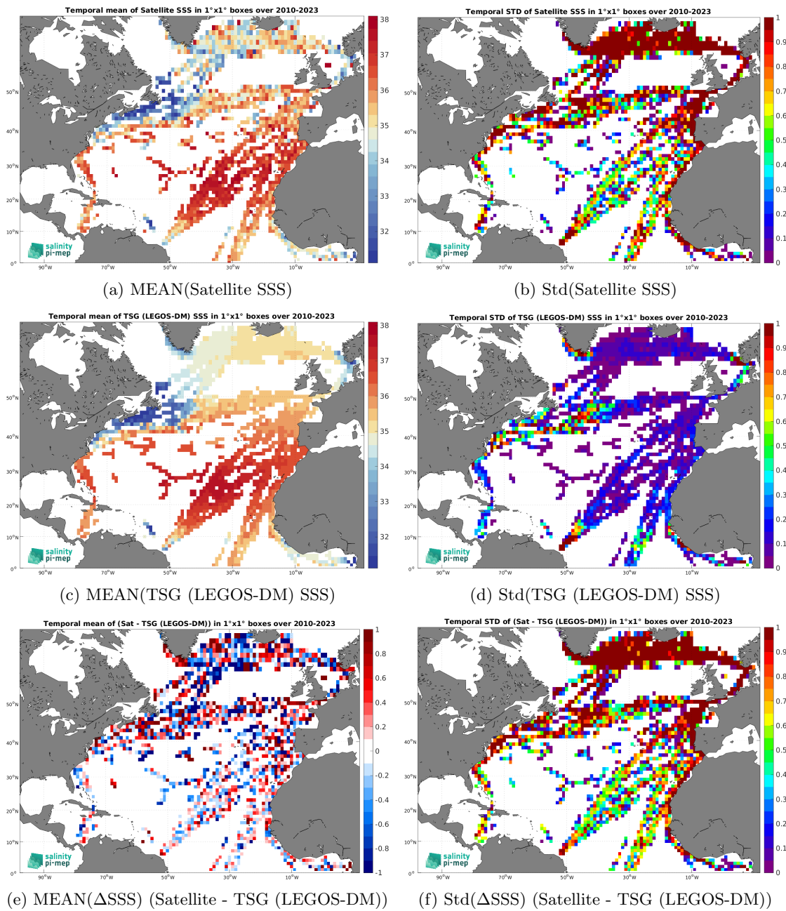
Figure 6: Temporal mean (left) and Std (right) of SSS from SMOS SSS L2Q v331 - 0.25 Deg (CATDS-CPDC) (top), TSG (LEGOS-DM) (middle), and of \Delta SSS (Satellite - TSG (LEGOS-DM)). Only match-up pairs are used to generate these maps.
