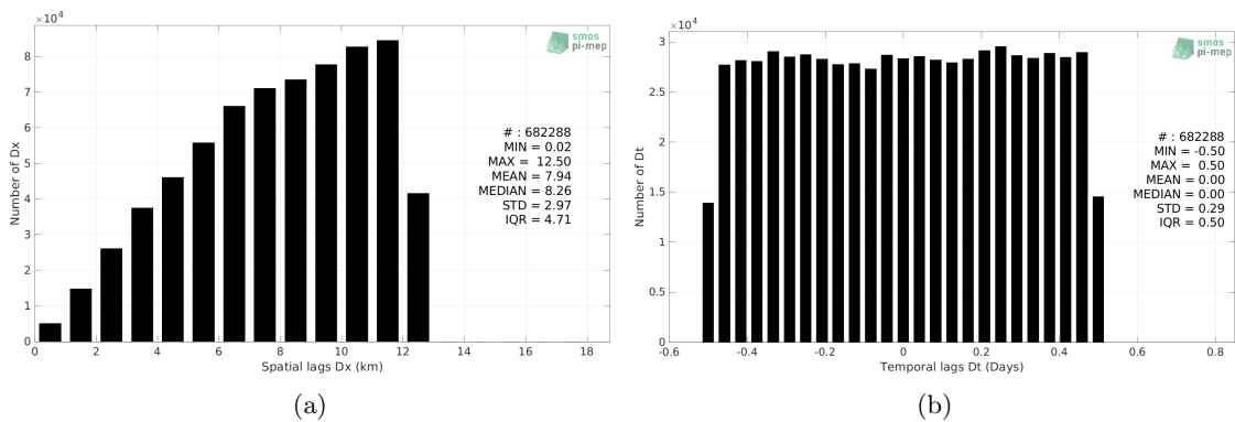
Figure 5: Histograms of the spatial (a) and temporal (b) lags between the location/time of the TSG (LEGOS-DM) measurement and the date of the corresponding SMOS SSS L2Q v331 - 0.25 Deg (CATDS-CPDC) SSS pixel.
