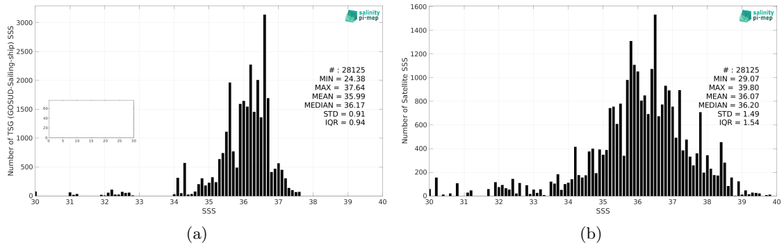
Figure 2: Histograms of SSS from TSG (GOSUD-Sailing-ship) (a) and SMOS SSS L2Q v331 - 0.25 Deg (CATDS-CPDC) (b) considering all match-up pairs per bins of 0.1 over the North Atlantic Ocean Pi-MEP region and for the full satellite product period.
