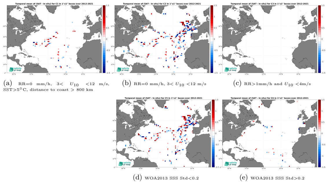
Figure 12: Temporal mean gridded over spatial boxes of size 1^\circ \times 1^\circ of \Delta\text{SSS} (SMOS SSS L2Q v331 - 0.25 Deg (CATDS-CPDC) - TSG (GOSUD-Sailing-ship)) for 5 different subdatasets corresponding to:RR=0 mm/h, 3 < U_{10} < 12 m/s, SST >5^\circ\text{C} , distance to coast > 800 km (a), RR=0 mm/h, 3 < U_{10} < 12 m/s (b), RR >1 mm/h and U_{10} < 4 m/s (c), WOA2013 SSS Std <0.2 (d), WOA2013 SSS Std >0.2 (e).
