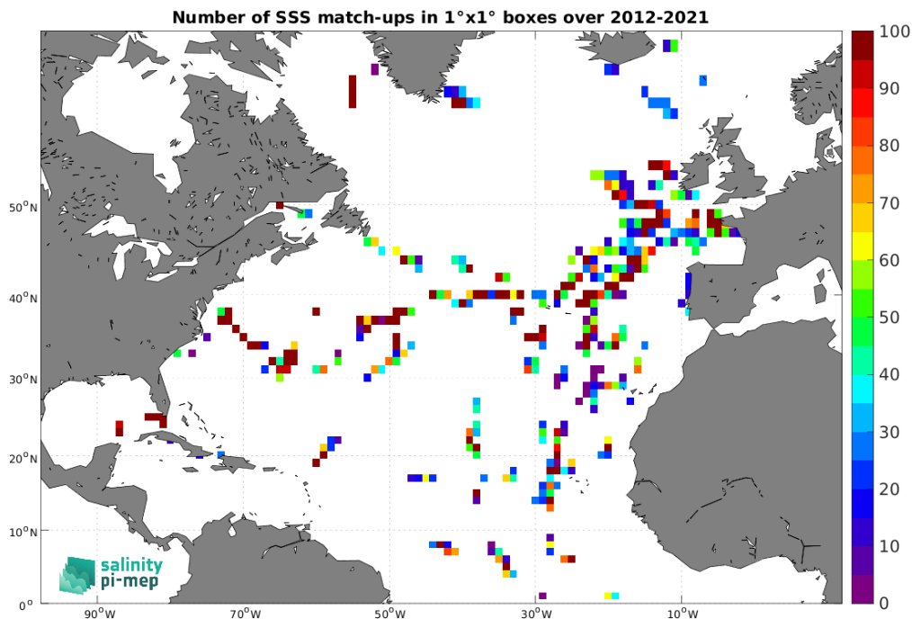
Figure 4: Number of SSS match-ups between TSG (GOSUD-Sailing-ship) SSS and the SMOS SSS L2Q v331 - 0.25 Deg (CATDS-CPDC) SSS product for the North Atlantic Ocean Pi-MEP region over 1^\circ \times 1^\circ boxes and for the full satellite product period.
