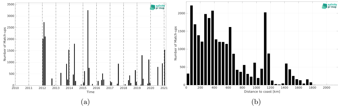
Figure 1: Number of match-ups between TSG (GOSUD-Sailing-ship) and SMOS SSS L2Q v331 - 0.25 Deg (CATDS-CPDC) SSS as a function of time (a) and as function of the distance to coast (b) over the North Atlantic Ocean Pi-MEP region and for the full satellite product period.
