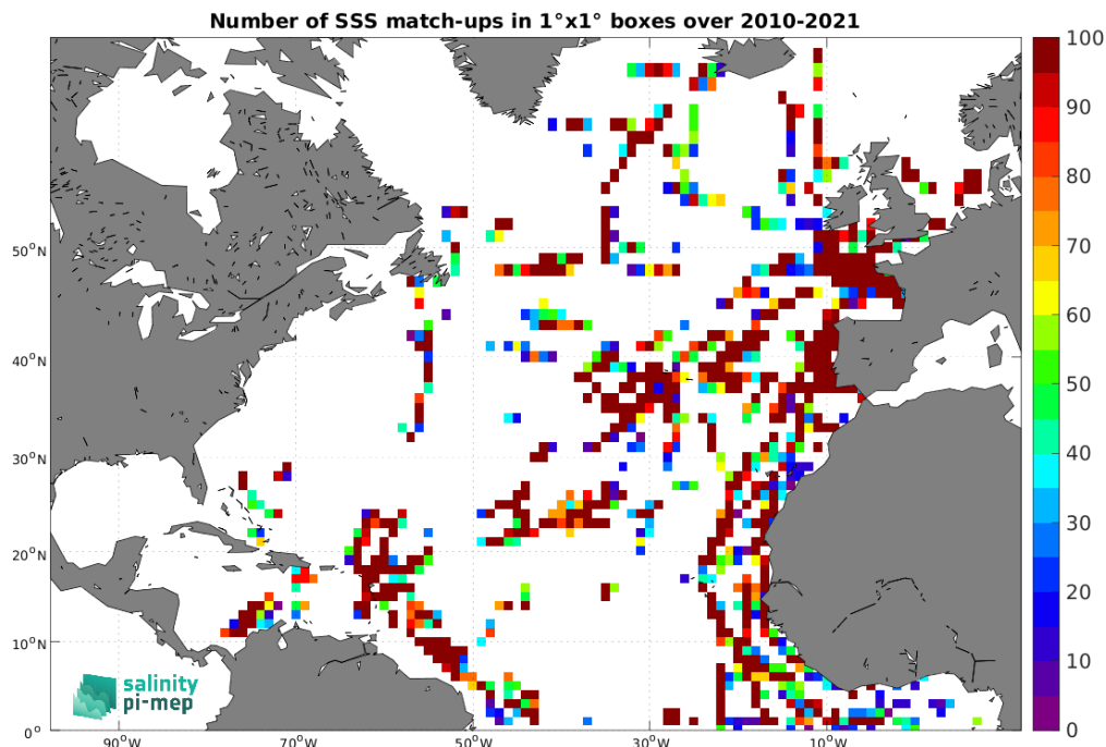
Figure 4: Number of SSS match-ups between TSG (GOSUD-Research-vessel) SSS and the SMOS SSS L2Q v331 - 0.25 Deg (CATDS-CPDC) SSS product for the North Atlantic Ocean Pi-MEP region over 1^\circ \times 1^\circ boxes and for the full satellite product period.
