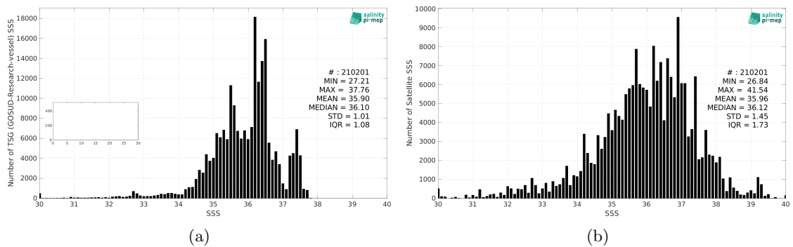
Figure 2: Histograms of SSS from TSG (GOSUD-Research-vessel) (a) and SMOS SSS L2Q v331 - 0.25 Deg (CATDS-CPDC) (b) considering all match-up pairs per bins of 0.1 over the North Atlantic Ocean Pi-MEP region and for the full satellite product period.
