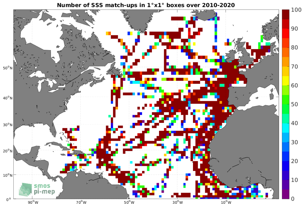
Figure 4: Number of SSS match-ups between TSG (GOSUD-Research-vessel) SSS and the SMOS SSS L2Q v331 - 0.25 Deg (CATDS-CPDC) SSS product for the North Atlantic Ocean Pi-MEP region over 1°×1° boxes and for the full satellite product period.
