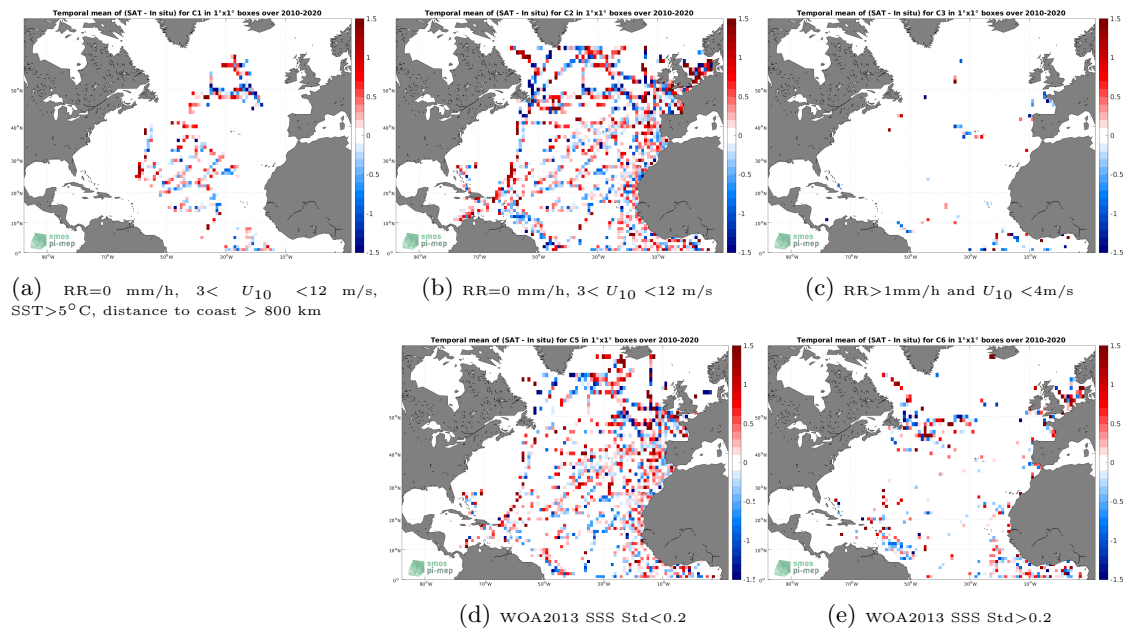
Figure 12: Temporal mean gridded over spatial boxes of size 1^\circ \times 1^\circ of \Delta\text{SSS} (SMOS SSS L2Q v331 - 0.25 Deg (CATDS-CPDC) - TSG (GOSUD-Research-vessel)) for 5 different subdatasets corresponding to:RR=0 mm/h, 3 < U_{10} < 12 m/s, SST >5^\circ\text{C} , distance to coast > 800 km (a), RR=0 mm/h, 3 < U_{10} < 12 m/s (b), RR >1 mm/h and U_{10} < 4 m/s (c), WOA2013 SSS Std <0.2 (d), WOA2013 SSS Std >0.2 (e).
