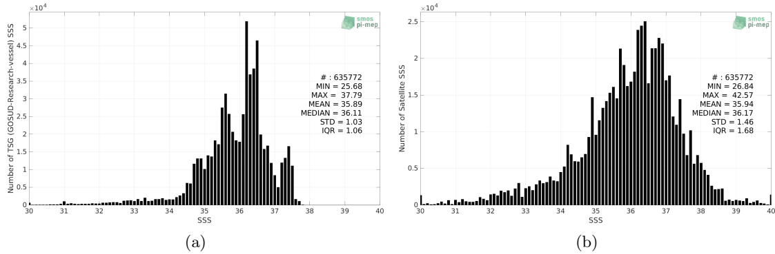
Figure 2: Histograms of SSS from TSG (GOSUD-Research-vessel) (a) and SMOS SSS L2Q v331 - 0.25 Deg (CATDS-CPDC) (b) considering all match-up pairs per bins of 0.1 over the North Atlantic Ocean Pi-MEP region and for the full satellite product period.
