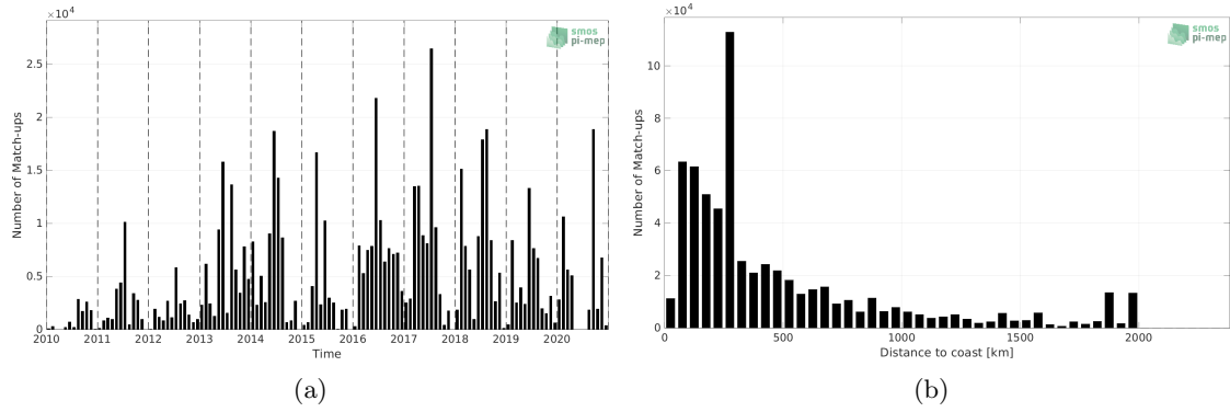
Figure 1: Number of match-ups between TSG (GOSUD-Research-vessel) and SMOS SSS L2Q v331 - 0.25 Deg (CATDS-CPDC) SSS as a function of time (a) and as function of the distance to coast (b) over the North Atlantic Ocean Pi-MEP region and for the full satellite product period.
