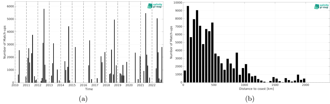
Figure 1: Number of match-ups between TSG (CSIC-UTM) and SMOS SSS L2Q v331 - 0.25 Deg (CATDS-CPDC) SSS as a function of time (a) and as function of the distance to coast (b) over the North Atlantic Ocean Pi-MEP region and for the full satellite product period.
