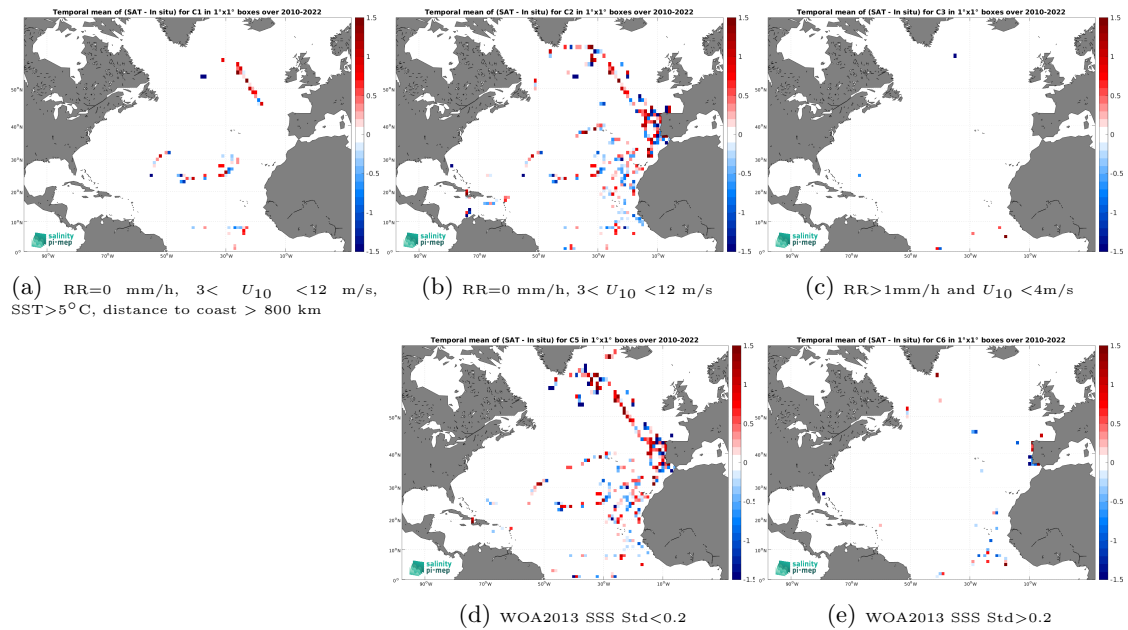
Figure 12: Temporal mean gridded over spatial boxes of size 1^\circ \times 1^\circ of \Delta\text{SSS} (SMOS SSS L2Q v331 - 0.25 Deg (CATDS-CPDC) - TSG (CSIC-UTM)) for 5 different subdatasets corresponding to:RR=0 mm/h, 3 < U_{10} < 12 m/s, SST >5^\circ\text{C} , distance to coast > 800 km (a), RR=0 mm/h, 3 < U_{10} < 12 m/s (b), RR >1 mm/h and U_{10} < 4 m/s (c), WOA2013 SSS Std <0.2 (d), WOA2013 SSS Std >0.2 (e).
