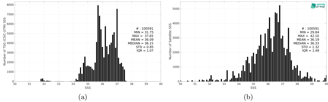
Figure 2: Histograms of SSS from TSG (CSIC-UTM) (a) and SMOS SSS L2Q v331 - 0.25 Deg (CATDS-CPDC) (b) considering all match-up pairs per bins of 0.1 over the North Atlantic Ocean Pi-MEP region and for the full satellite product period.
