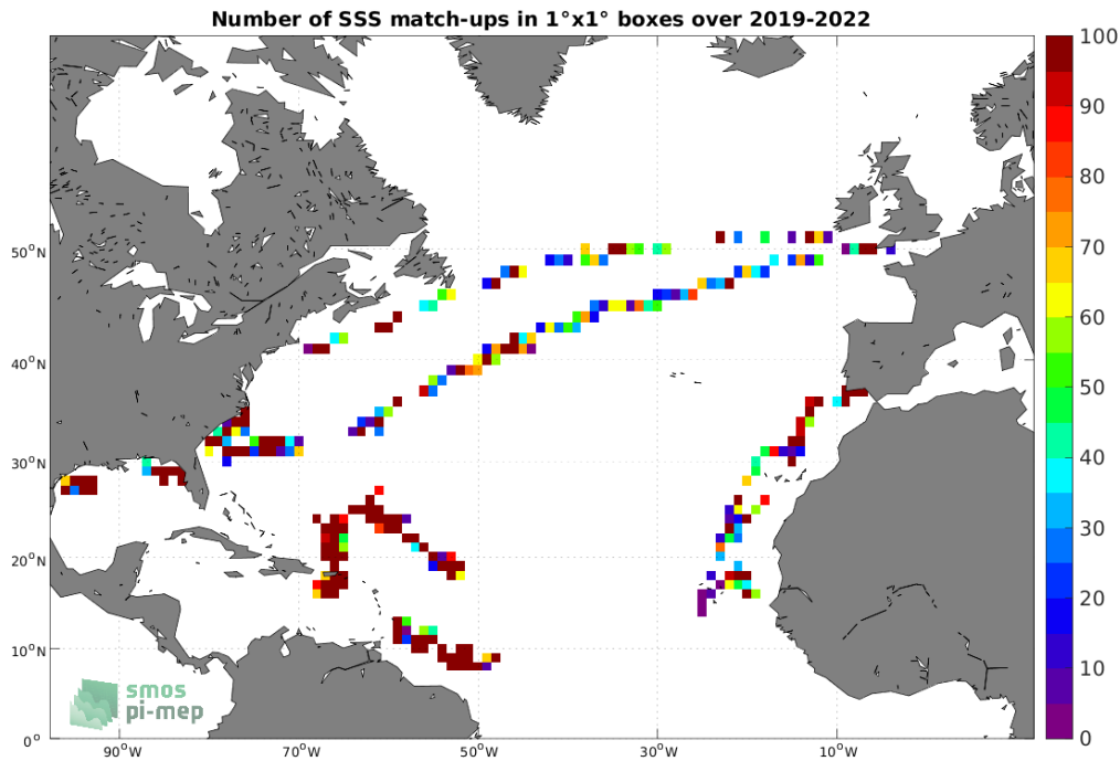
Figure 4: Number of SSS match-ups between Saildrone SSS and the SMOS SSS L2Q v331 - 0.25 Deg (CATDS-CPDC) SSS product for the North Atlantic Ocean Pi-MEP region over 1^\circ \times 1^\circ boxes and for the full satellite product period.
