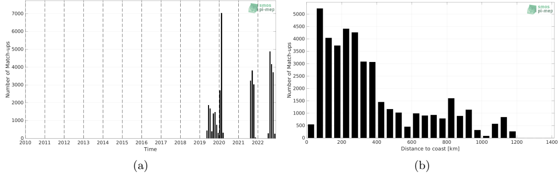
Figure 1: Number of match-ups between Saildrone and SMOS SSS L2Q v331 - 0.25 Deg (CATDS-CPDC) SSS as a function of time (a) and as function of the distance to coast (b) over the North Atlantic Ocean Pi-MEP region and for the full satellite product period.
