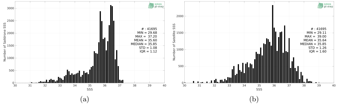
Figure 2: Histograms of SSS from Saildrone (a) and SMOS SSS L2Q v331 - 0.25 Deg (CATDS-CPDC) (b) considering all match-up pairs per bins of 0.1 over the North Atlantic Ocean Pi-MEP region and for the full satellite product period.
