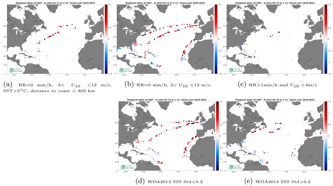
Figure 12: Temporal mean gridded over spatial boxes of size 1^\circ \times 1^\circ of \Delta\text{SSS} (SMOS SSS L2Q v331 - 0.25 Deg (CATDS-CPDC) - Saildrone) for 5 different subdatasets corresponding to:RR=0 mm/h, 3 < U_{10} < 12 m/s, SST > 5^\circ\text{C} , distance to coast > 800 km (a), RR=0 mm/h, 3 < U_{10} < 12 m/s (b), RR > 1 mm/h and U_{10} < 4 m/s (c), WOA2013 SSS Std < 0.2 (d), WOA2013 SSS Std > 0.2 (e).
