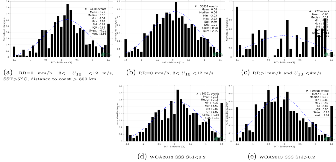
Figure 13: Normalized histogram of \Delta SSS (SMOS SSS L2Q v331 - 0.25 Deg (CATDS-CPDC) - Sairdronne) for 5 different subdatasets corresponding to: RR=0 mm/h, 3 < U_{10} < 12 m/s, SST > 5°C, distance to coast > 800 km (a), RR=0 mm/h, 3 < U_{10} < 12 m/s (b), RR > 1mm/h and U_{10} < 4 m/s (c), WOA2013 SSS Std < 0.2 (d), WOA2013 SSS Std > 0.2 (e).
