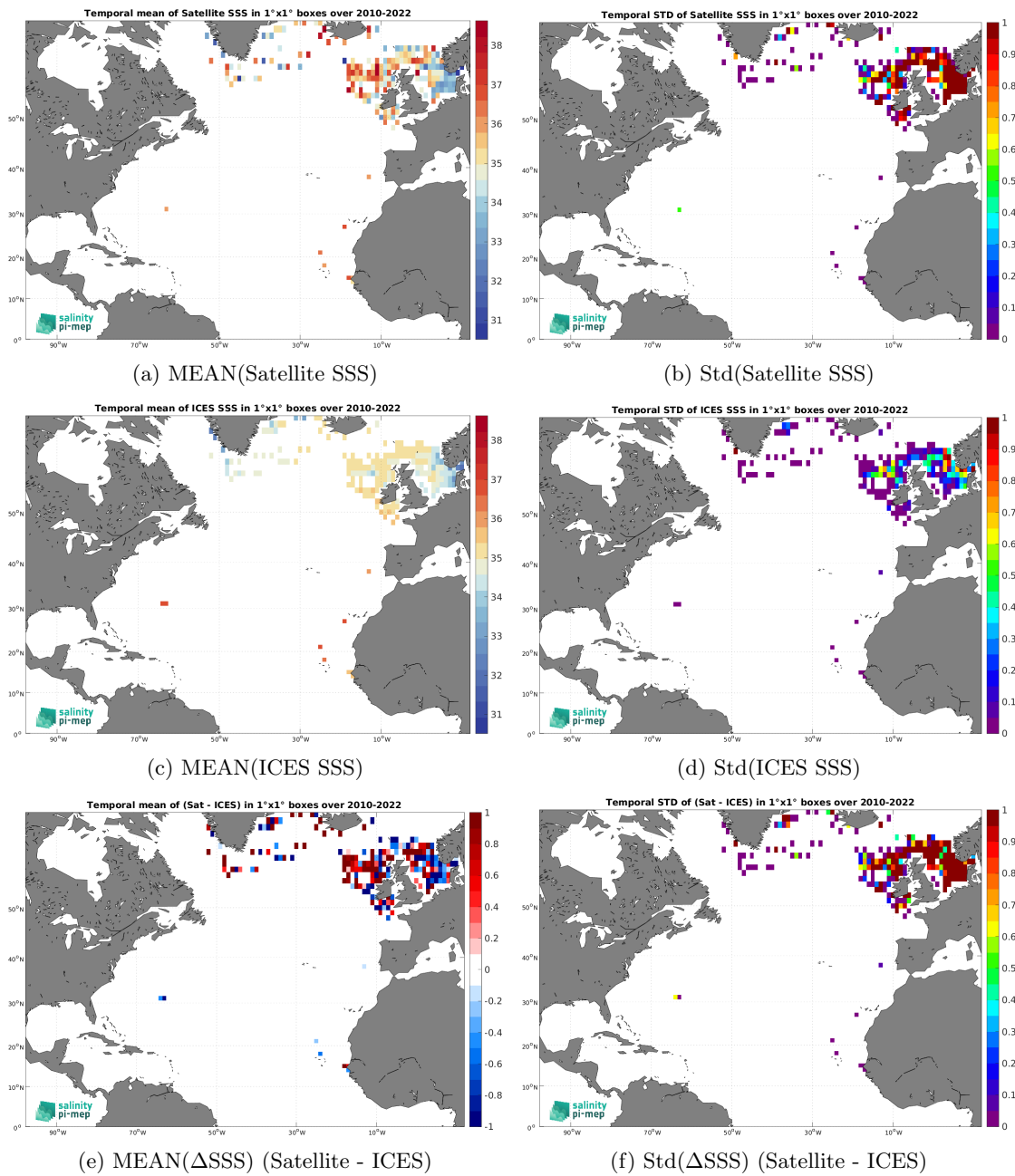
Figure 6: Temporal mean (left) and Std (right) of SSS from SMOS SSS L2Q v331 - 0.25 Deg (CATDS-CPDC) (top), ICES (middle), and of \Delta SSS (Satellite - ICES). Only match-up pairs are used to generate these maps.
