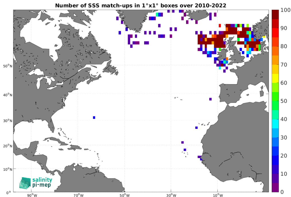
Figure 4: Number of SSS match-ups between ICES SSS and the SMOS SSS L2Q v331 - 0.25 Deg (CATDS-CPDC) SSS product for the North Atlantic Ocean Pi-MEP region over 1^\circ \times 1^\circ boxes and for the full satellite product period.
