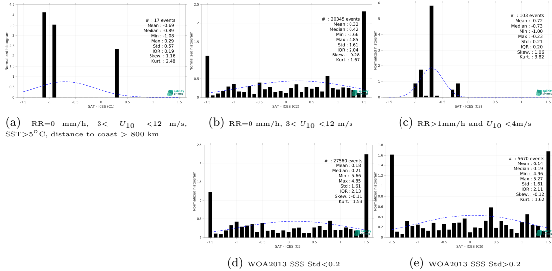
Figure 13: Normalized histogram of \Delta SSS (SMOS SSS L2Q v331 - 0.25 Deg (CATDS-CPDC) - ICES) for 5 different subdatasets corresponding to: RR=0 mm/h, 3 < U_{10} < 12 m/s, SST>5°C, distance to coast > 800 km (a), RR=0 mm/h, 3 < U_{10} < 12 m/s (b), RR>1mm/h and U_{10} < 4 m/s (c), WOA2013 SSS Std<0.2 (d), WOA2013 SSS Std>0.2 (e).
