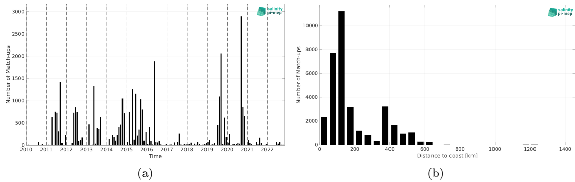
Figure 1: Number of match-ups between ICES and SMOS SSS L2Q v331 - 0.25 Deg (CATDS-CPDC) SSS as a function of time (a) and as function of the distance to coast (b) over the North Atlantic Ocean Pi-MEP region and for the full satellite product period.
