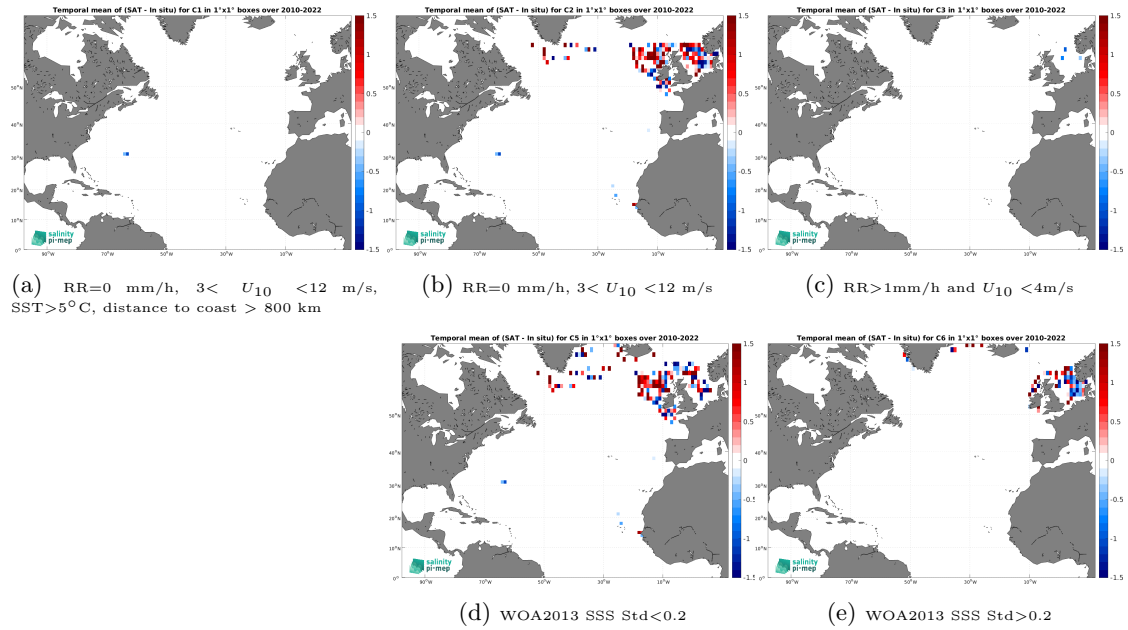
Figure 12: Temporal mean gridded over spatial boxes of size 1^\circ \times 1^\circ of \Delta\text{SSS} (SMOS SSS L2Q v331 - 0.25 Deg (CATDS-CPDC) - ICES) for 5 different subdatasets corresponding to:RR=0 mm/h, 3 < U_{10} < 12 m/s, SST >5^\circ\text{C} , distance to coast > 800 km (a), RR=0 mm/h, 3 < U_{10} < 12 m/s (b), RR >1 mm/h and U_{10} < 4 m/s (c), WOA2013 SSS Std <0.2 (d), WOA2013 SSS Std >0.2 (e).
