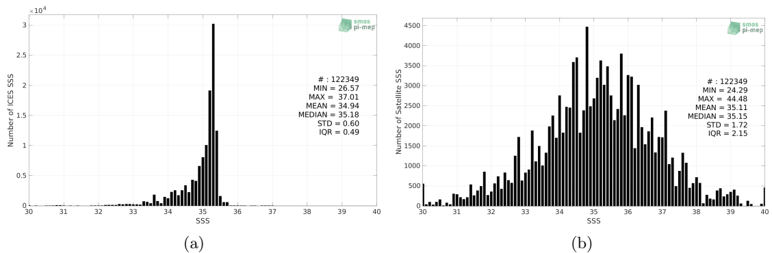
Figure 2: Histograms of SSS from ICES (a) and SMOS SSS L2Q v331 - 0.25 Deg (CATDS-CPDC) (b) considering all match-up pairs per bins of 0.1 over the North Atlantic Ocean Pi-MEP region and for the full satellite product period.
