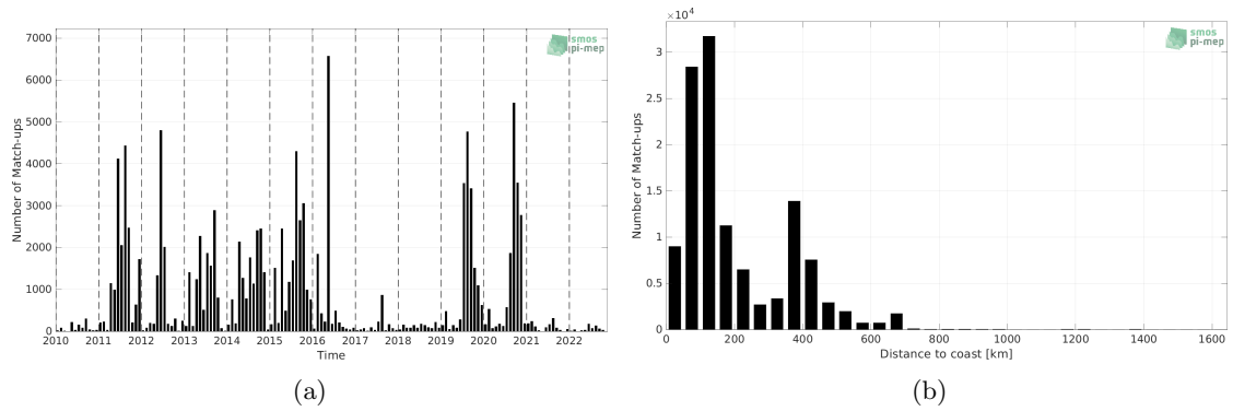
Figure 1: Number of match-ups between ICES and SMOS SSS L2Q v331 - 0.25 Deg (CATDS-CPDC) SSS as a function of time (a) and as function of the distance to coast (b) over the North Atlantic Ocean Pi-MEP region and for the full satellite product period.
