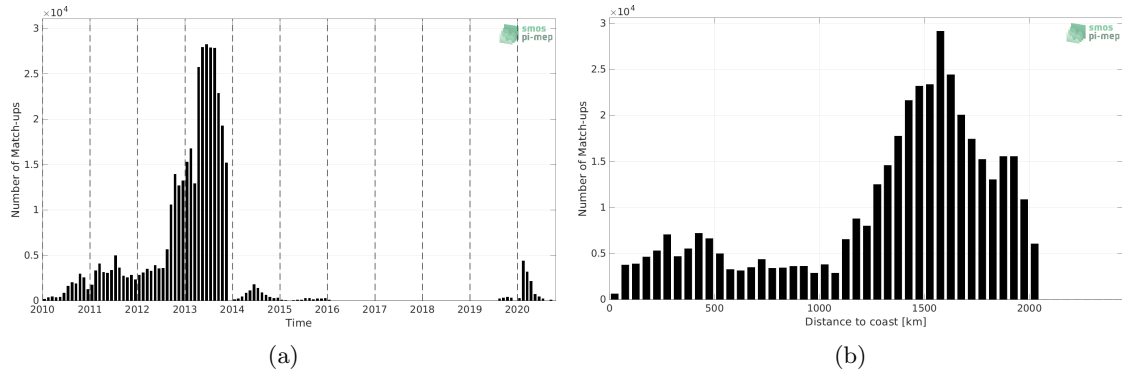
Figure 1: Number of match-ups between Surface drifters and SMOS SSS L2Q v331 - 0.25 Deg (CATDS-CPDC) SSS as a function of time (a) and as function of the distance to coast (b) over the North Atlantic Ocean Pi-MEP region and for the full satellite product period.
