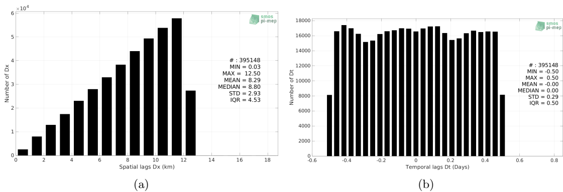
Figure 4: Histograms of the spatial (a) and temporal (b) lags between the location/time of the Surface drifters measurement and the date of the corresponding SMOS SSS L2Q v331 - 0.25 Deg (CATDS-CPDC) SSS pixel.
