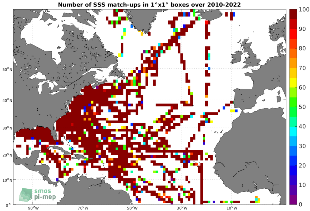
Figure 4: Number of SSS match-ups between TSG (SAMOS) SSS and the SMOS SSS L2Q v330 - 0.25 Deg (CATDS-CPDC) SSS product for the North Atlantic Ocean Pi-MEP region over 1^\circ \times 1^\circ boxes and for the full satellite product period.
