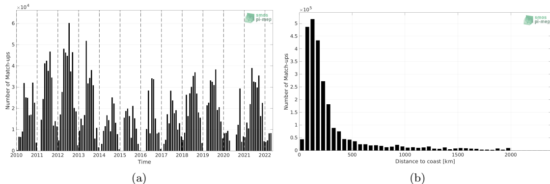
Figure 1: Number of match-ups between TSG (SAMOS) and SMOS SSS L2Q v330 - 0.25 Deg (CATDS-CPDC) SSS as a function of time (a) and as function of the distance to coast (b) over the North Atlantic Ocean Pi-MEP region and for the full satellite product period.
