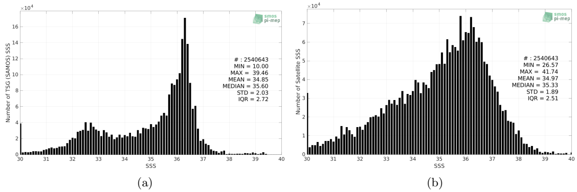
Figure 2: Histograms of SSS from TSG (SAMOS) (a) and SMOS SSS L2Q v330 - 0.25 Deg (CATDS-CPDC) (b) considering all match-up pairs per bins of 0.1 over the North Atlantic Ocean Pi-MEP region and for the full satellite product period.
