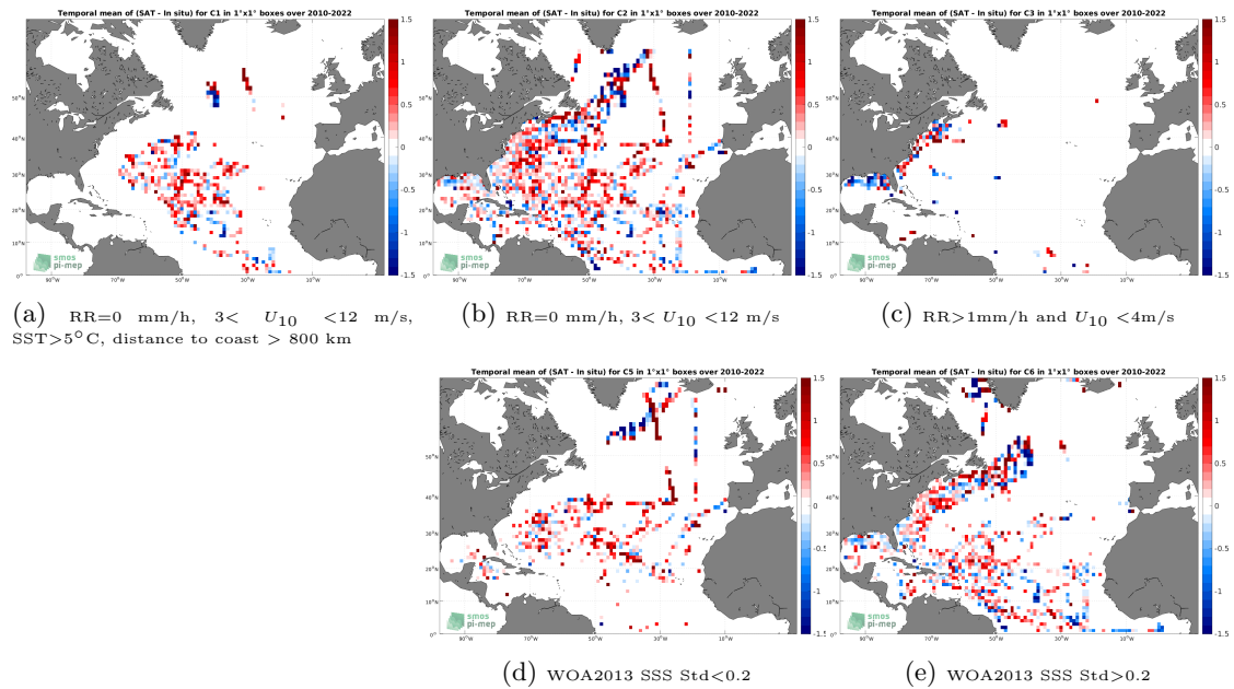
Figure 12: Temporal mean gridded over spatial boxes of size 1^\circ \times 1^\circ of \Delta\text{SSS} (SMOS SSS L2Q v330 - 0.25 Deg (CATDS-CPDC) - TSG (SAMOS)) for 5 different subdatasets corresponding to:RR=0 mm/h, 3 < U_{10} < 12 m/s, SST >5^\circ\text{C} , distance to coast > 800 km (a), RR=0 mm/h, 3 < U_{10} < 12 m/s (b), RR >1 mm/h and U_{10} < 4 m/s (c), WOA2013 SSS Std <0.2 (d), WOA2013 SSS Std >0.2 (e).
