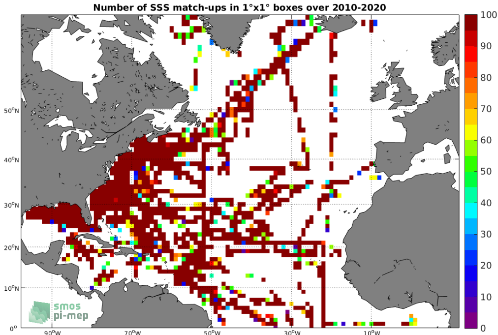
Figure 4: Number of SSS match-ups between TSG (SAMOS) SSS and the SMOS SSS L2Q v330 - 0.25 Deg (CATDS-CPDC) SSS product for the North Atlantic Ocean Pi-MEP region over 1^{\circ} \times 1^{\circ} boxes and for the full satellite product period.
