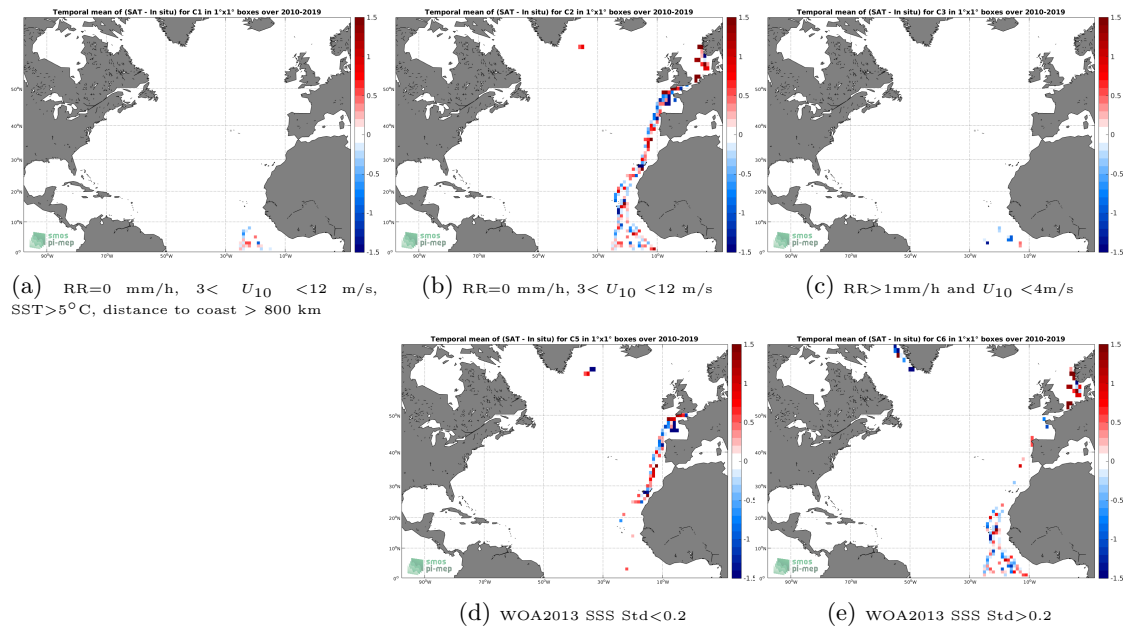
Figure 12: Temporal mean gridded over spatial boxes of size 1^\circ \times 1^\circ of \Delta\text{SSS} (SMOS SSS L2Q v330 - 0.25 Deg (CATDS-CPDC) - TSG (Polarstern)) for 5 different subdatasets corresponding to:RR=0 mm/h, 3 < U_{10} < 12 m/s, SST >5^\circ\text{C} , distance to coast > 800 km (a), RR=0 mm/h, 3 < U_{10} < 12 m/s (b), RR >1 mm/h and U_{10} < 4 m/s (c), WOA2013 SSS Std <0.2 (d), WOA2013 SSS Std >0.2 (e).
