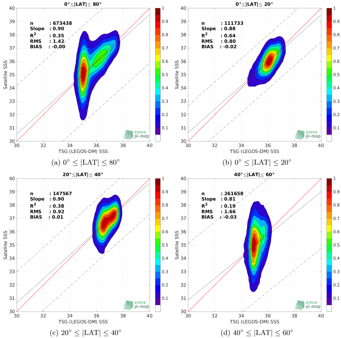
Figure 9: Contour maps of the concentration of SMOS SSS L2Q v330 - 0.25 Deg (CATDS-CPDC) SSS ( y -axis) versus TSG (LEGOS-DM) SSS ( x -axis) at match-up pairs for different latitude bands. For each plot, the red line shows x=y . The black thin and dashed lines indicate a linear fit through the data cloud and the \pm 95\% confidence levels, respectively. The number match-up pairs n , the slope and R^2 coefficient of the linear fit, the root mean square (RMS) and the mean bias between satellite and in situ data are indicated for each latitude band in each plots.
