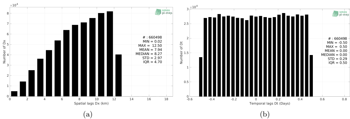
Figure 5: Histograms of the spatial (a) and temporal (b) lags between the location/time of the TSG (LEGOS-DM) measurement and the date of the corresponding SMOS SSS L2Q v330 - 0.25 Deg (CATDS-CPDC) SSS pixel.
