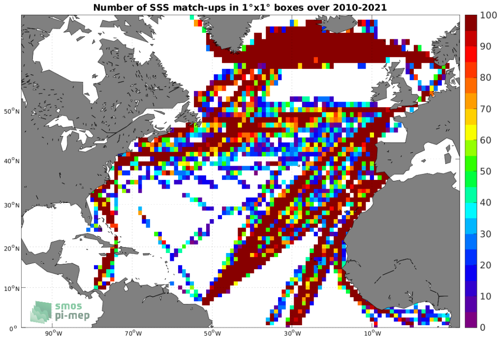
Figure 4: Number of SSS match-ups between TSG (LEGOS-DM) SSS and the SMOS SSS L2Q v330 - 0.25 Deg (CATDS-CPDC) SSS product for the North Atlantic Ocean Pi-MEP region over 1^\circ \times 1^\circ boxes and for the full satellite product period.
