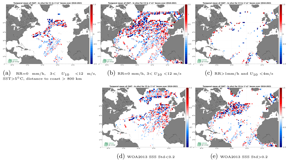
Figure 12: Temporal mean gridded over spatial boxes of size 1^\circ \times 1^\circ of \Delta\text{SSS} (SMOS SSS L2Q v330 - 0.25 Deg (CATDS-CPDC) - TSG (LEGOS-DM)) for 5 different subdatasets corresponding to:RR=0 mm/h, 3 < U_{10} < 12 m/s, SST >5^\circ\text{C} , distance to coast > 800 km (a), RR=0 mm/h, 3 < U_{10} < 12 m/s (b), RR >1 mm/h and U_{10} < 4 m/s (c), WOA2013 SSS Std <0.2 (d), WOA2013 SSS Std >0.2 (e).
