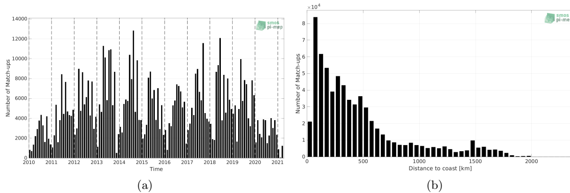
Figure 1: Number of match-ups between TSG (LEGOS-DM) and SMOS SSS L2Q v330 - 0.25 Deg (CATDS-CPDC) SSS as a function of time (a) and as function of the distance to coast (b) over the North Atlantic Ocean Pi-MEP region and for the full satellite product period.
