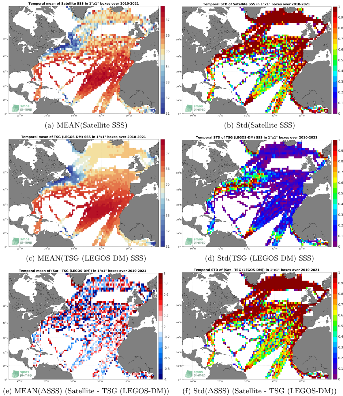
Figure 6: Temporal mean (left) and Std (right) of SSS from SMOS SSS L2Q v330 - 0.25 Deg (CATDS-CPDC) (top), TSG (LEGOS-DM) (middle), and of \Delta SSS (Satellite - TSG (LEGOS-DM)). Only match-up pairs are used to generate these maps.
