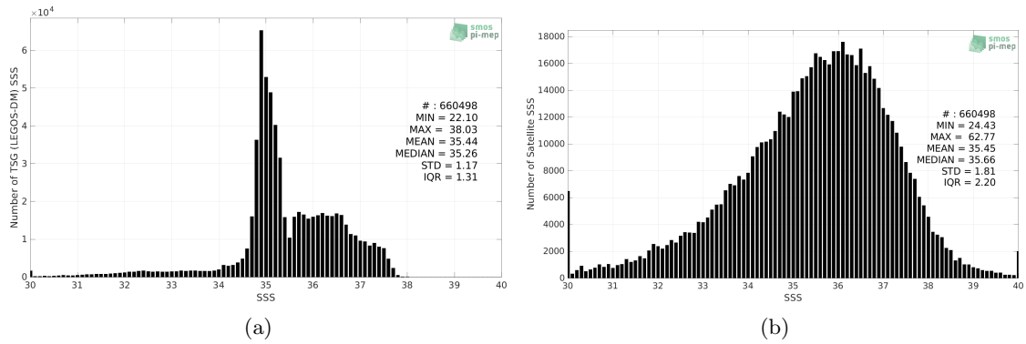
Figure 2: Histograms of SSS from TSG (LEGOS-DM) (a) and SMOS SSS L2Q v330 - 0.25 Deg (CATDS-CPDC) (b) considering all match-up pairs per bins of 0.1 over the North Atlantic Ocean Pi-MEP region and for the full satellite product period.
