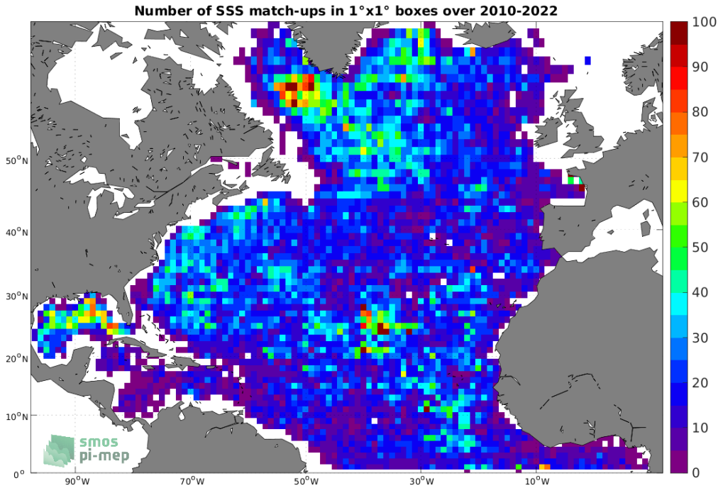
Figure 4: Number of SSS match-ups between Argo SSS and the SMOS SSS L2Q v330 - 0.25 Deg (CATDS-CPDC) SSS product for the North Atlantic Ocean Pi-MEP region over 1^{\circ} \times 1^{\circ} boxes and for the full satellite product period.
