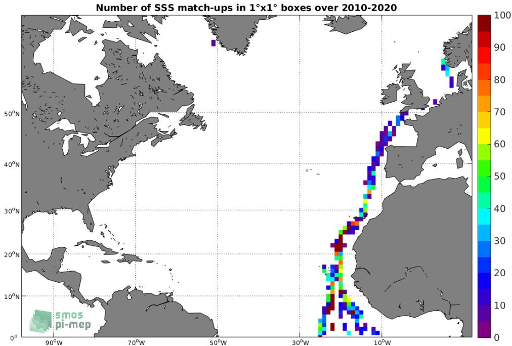
Figure 4: Number of SSS match-ups between TSG (Polarstern) SSS and the SMOS SSS L2Q v321 - 0.25 Deg (CATDS-CPDC) SSS product for the North Atlantic Ocean Pi-MEP region over 1^\circ \times 1^\circ boxes and for the full satellite product period.
