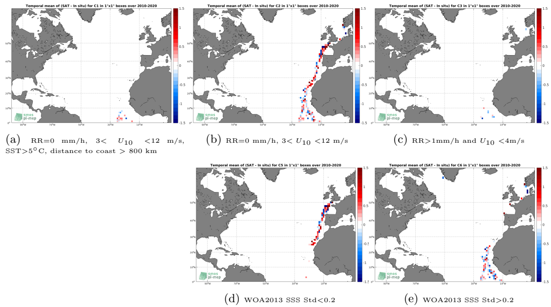
Figure 12: Temporal mean gridded over spatial boxes of size 1^\circ \times 1^\circ of \Delta\text{SSS} (SMOS SSS L2Q v321 - 0.25 Deg (CATDS-CPDC) - TSG (Polarstern)) for 5 different subdatasets corresponding to:RR=0 mm/h, 3 < U_{10} < 12 m/s, SST > 5^\circ\text{C} , distance to coast > 800 km (a), RR=0 mm/h, 3 < U_{10} < 12 m/s (b), RR > 1 mm/h and U_{10} < 4 m/s (c), WOA2013 SSS Std < 0.2 (d), WOA2013 SSS Std > 0.2 (e).
