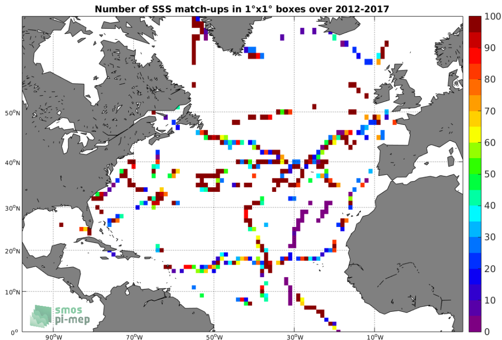
Figure 4: Number of SSS match-ups between TSG-GOSUD-Sailing-ship SSS and the SMOS L2Q v321 - 0.25 Deg (CATDS-CPDC) SSS product for the North Atlantic Ocean Pi-MEP region over 1^\circ \times 1^\circ boxes and for the full satellite product period.
