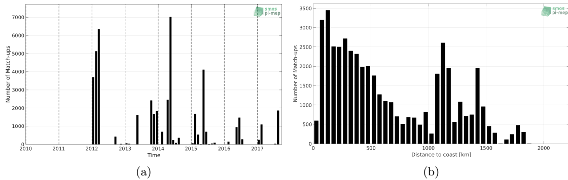
Figure 1: Number of match-ups between TSG-GOSUD-Sailing-ship and SMOS L2Q v321 - 0.25 Deg (CATDS-CPDC) SSS as a function of time (a) and as function of the distance to coast (b) over the North Atlantic Ocean Pi-MEP region and for the full satellite product period.
