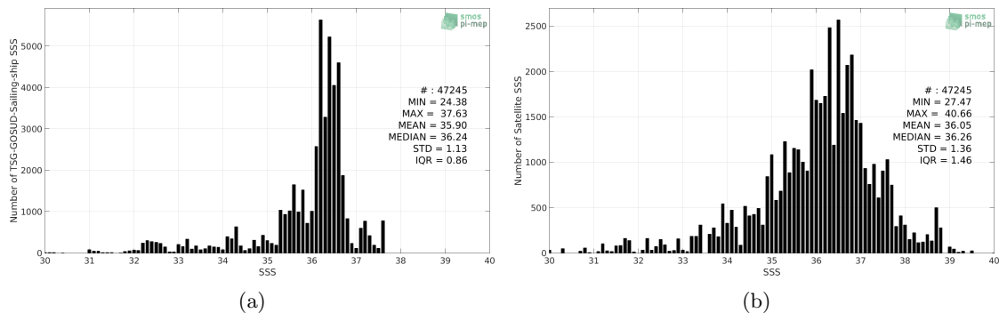
Figure 2: Histograms of SSS from TSG-GOSUD-Sailing-ship (a) and SMOS L2Q v321 - 0.25 Deg (CATDS-CPDC) (b) considering all match-up pairs per bins of 0.1 over the North Atlantic Ocean Pi-MEP region and for the full satellite product period.
