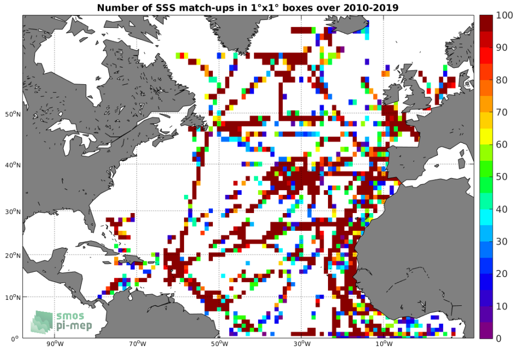
Figure 4: Number of SSS match-ups between TSG (GOSUD-Research-vessel) SSS and the SMOS SSS L2Q v321 - 0.25 Deg (CATDS-CPDC) SSS product for the North Atlantic Ocean Pi-MEP region over 1^{\circ} \times 1^{\circ} boxes and for the full satellite product period.
