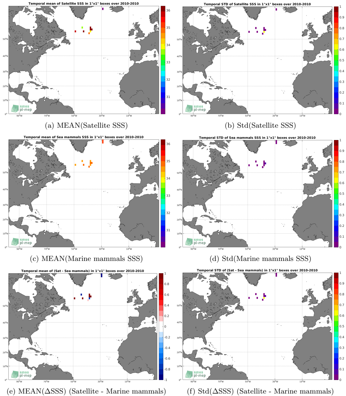
Figure 6: Temporal mean (left) and Std (right) of SSS from SMOS SSS L2Q v321 - 0.25 Deg (CATDS-CPDC) (top), Marine mammals (middle), and of \Delta SSS (Satellite - Marine mammals). Only match-up pairs are used to generate these maps.
