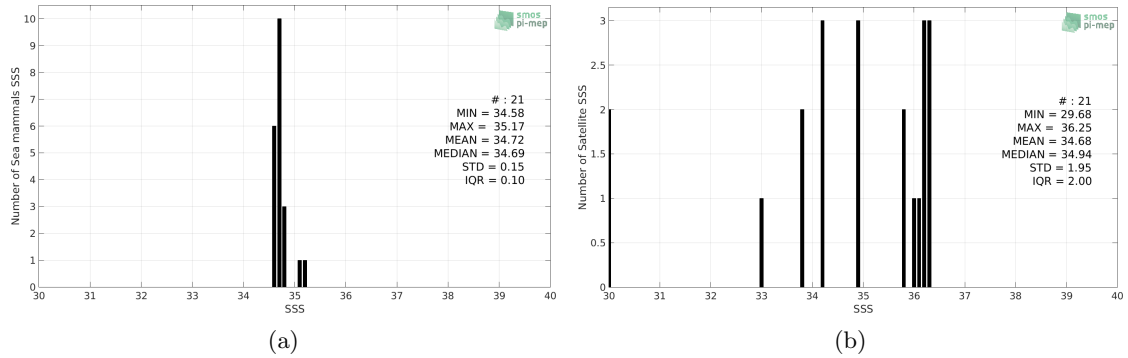
Figure 2: Histograms of SSS from Marine mammals (a) and SMOS SSS L2Q v321 - 0.25 Deg (CATDS-CPDC) (b) considering all match-up pairs per bins of 0.1 over the North Atlantic Ocean Pi-MEP region and for the full satellite product period.
