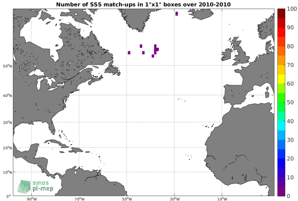
Figure 4: Number of SSS match-ups between Marine mammals SSS and the SMOS SSS L2Q v321 - 0.25 Deg (CATDS-CPDC) SSS product for the North Atlantic Ocean Pi-MEP region over 1^\circ \times 1^\circ boxes and for the full satellite product period.
