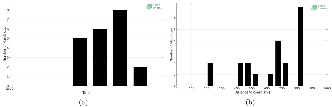
Figure 1: Number of match-ups between Marine mammals and SMOS SSS L2Q v321 - 0.25 Deg (CATDS-CPDC) SSS as a function of time (a) and as function of the distance to coast (b) over the North Atlantic Ocean Pi-MEP region and for the full satellite product period.
