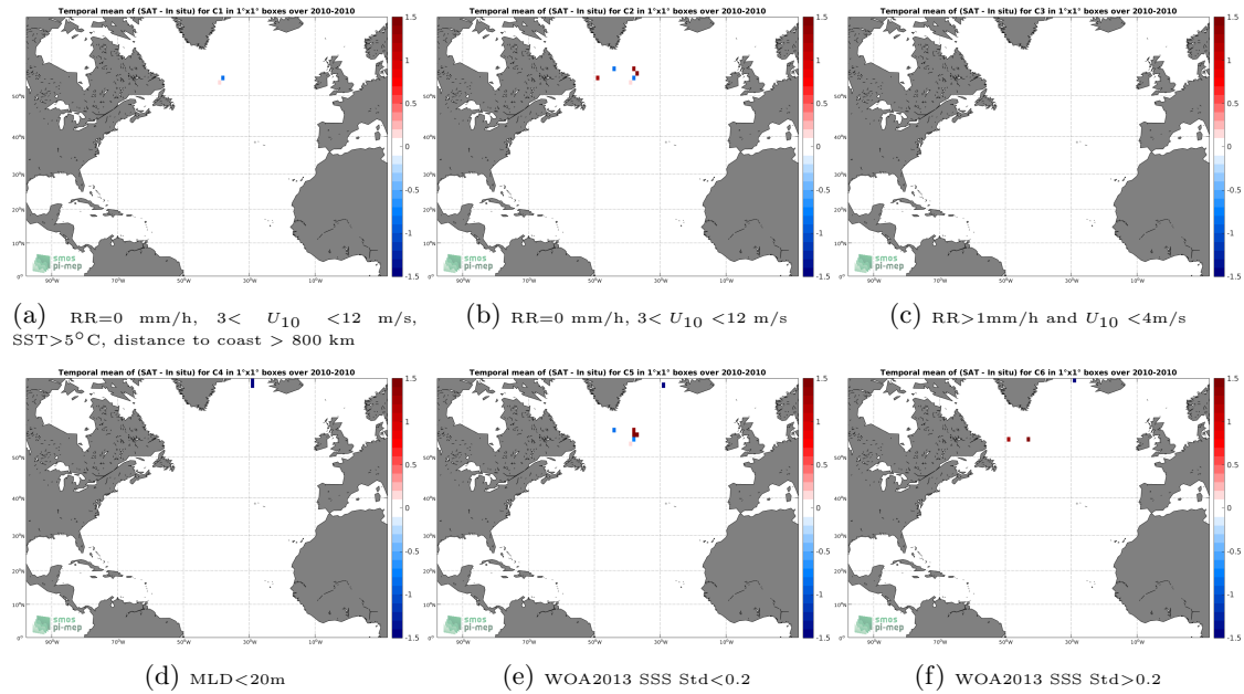
Figure 12: Temporal mean gridded over spatial boxes of size 1^{\circ}\times 1^{\circ} of \Delta\text{SSS} (SMOS SSS L2Q v321 - 0.25 Deg (CATDS-CPDC) - Marine mammals) for 6 different subdatasets corresponding to:RR=0 mm/h, 3 < U_{10} < 12 m/s, SST > 5^{\circ}\text{C} , distance to coast > 800 km (a), RR=0 mm/h, 3 < U_{10} < 12 m/s (b), RR > 1\text{mm/h} and U_{10} < 4\text{m/s} (c),MLD < 20\text{m} (d),WOA2013 SSS Std < 0.2 (e),WOA2013 SSS Std > 0.2 (f).
