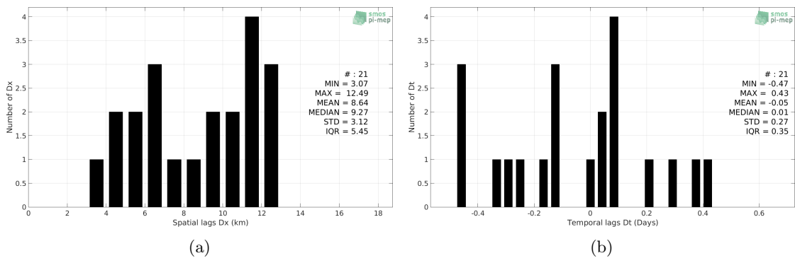
Figure 5: Histograms of the spatial (a) and temporal (b) lags between the location/time of the Marine mammals measurement and the date of the corresponding SMOS SSS L2Q v321 - 0.25 Deg (CATDS-CPDC) SSS pixel.
