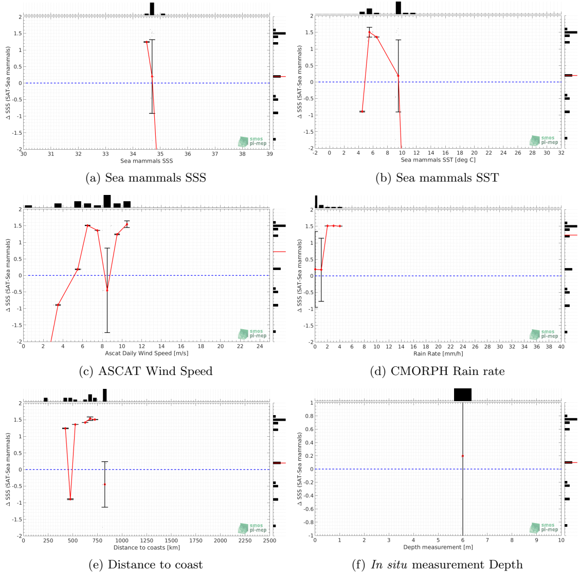
Figure 11: \Delta \text{SSS} (Satellite - Sea mammals) sorted as function of Sea mammals SSS a), Sea mammals SST b), ASCAT Wind speed c), CMORPH rain rate d), distance to coast (e) and in situ measurement depth (f). In all plots the median and Std of \Delta \text{SSS} for each bin is indicated by the red curves and black vertical thick bars ( \pm 1 Std)
