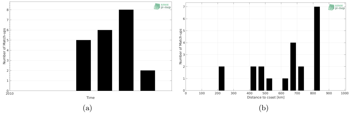
Figure 1: Number of match-ups between Sea mammals and SMOS SSS L2Q v321 - 0.25 Deg (CATDS-CPDC) SSS as a function of time (a) and as function of the distance to coast (b) over the North Atlantic Ocean Pi-MEP region and for the full satellite product period.
