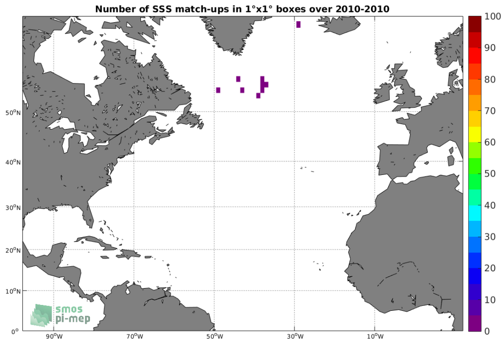
Figure 4: Number of SSS match-ups between Sea mammals SSS and the SMOS SSS L2Q v321 - 0.25 Deg (CATDS-CPDC) SSS product for the North Atlantic Ocean Pi-MEP region over 1°x1° boxes and for the full satellite product period.
