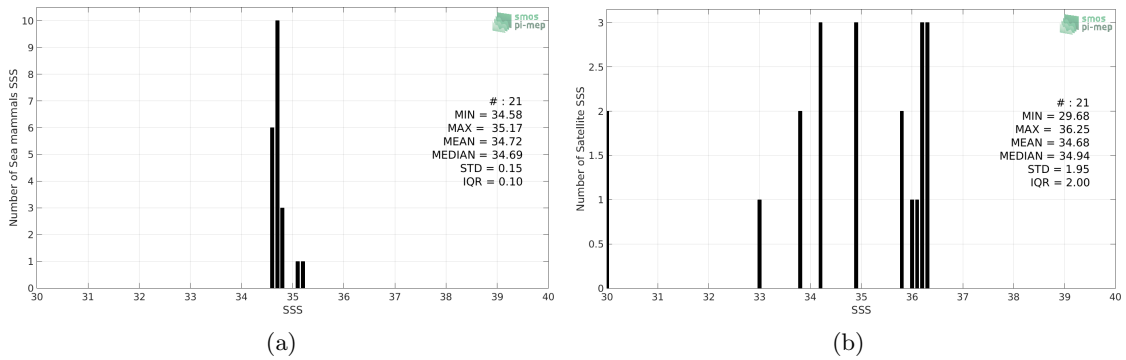
Figure 2: Histograms of SSS from Sea mammals (a) and SMOS SSS L2Q v321 - 0.25 Deg (CATDS-CPDC) (b) considering all match-up pairs per bins of 0.1 over the North Atlantic Ocean Pi-MEP region and for the full satellite product period.
