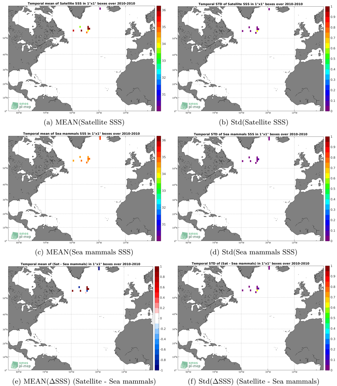
Figure 6: Temporal mean (left) and Std (right) of SSS from SMOS SSS L2Q v321 - 0.25 Deg (CATDS-CPDC) (top), Sea mammals (middle), and of \Delta SSS (Satellite - Sea mammals). Only match-up pairs are used to generate these maps.
