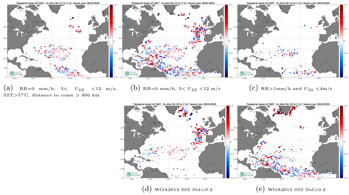
Figure 11: Temporal mean gridded over spatial boxes of size 1^\circ \times 1^\circ of \Delta\text{SSS} (SMOS SSS L2Q v321 - 0.25 Deg (CATDS-CPDC) - Surface drifters) for 5 different subdatasets corresponding to:RR=0 mm/h, 3 < U_{10} < 12 m/s, SST>5°C, distance to coast > 800 km (a), RR=0 mm/h, 3 < U_{10} < 12 m/s (b), RR>1mm/h and U_{10} < 4 m/s (c), WOA2013 SSS Std<0.2 (d), WOA2013 SSS Std>0.2 (e).
