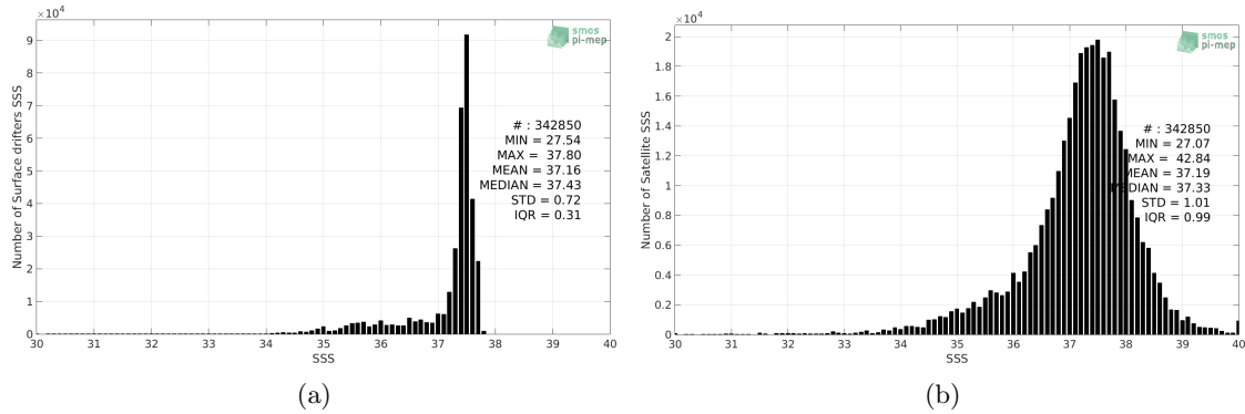
Figure 2: Histograms of SSS from Surface drifters (a) and SMOS L2Q v321 - 0.25 Deg (CATDS-CPDC) (b) considering all match-up pairs per bins of 0.1 over the North Atlantic Ocean Pi-MEP region and for the full satellite product period.
