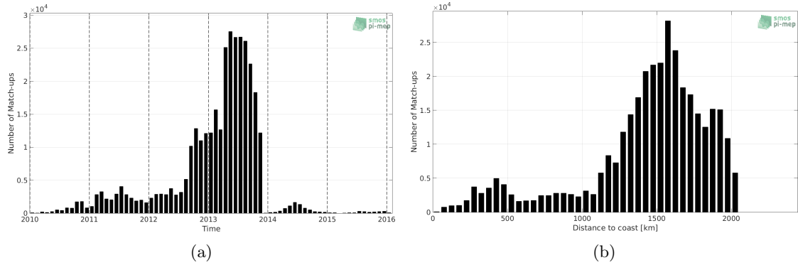
Figure 1: Number of match-ups between Surface drifters and SMOS L2Q v321 - 0.25 Deg (CATDS-CPDC) SSS as a function of time (a) and as function of the distance to coast (b) over the North Atlantic Ocean Pi-MEP region and for the full satellite product period.
