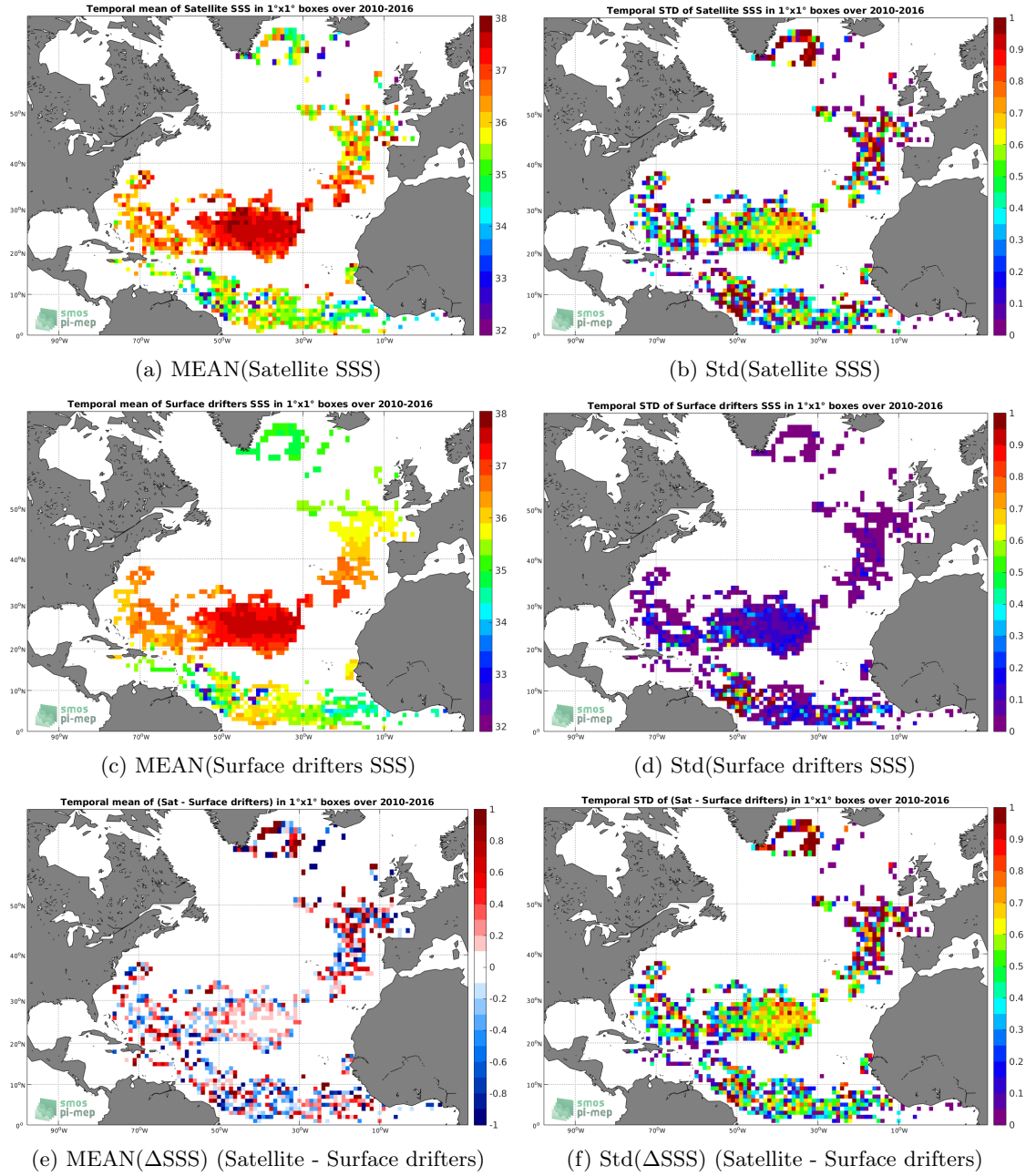
Figure 5: Temporal mean (left) and Std (right) of SSS from SMOS L2Q v321 - 0.25 Deg (CATDS-CPDC) (top), Surface drifters (middle), and of \Delta SSS (Satellite - Surface drifters). Only match-up pairs are used to generate these maps.
