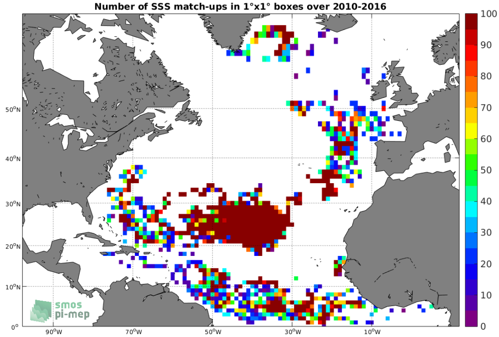
Figure 3: Number of SSS match-ups between Surface drifters SSS and the SMOS L2Q v321 - 0.25 Deg (CATDS-CPDC) SSS product for the North Atlantic Ocean Pi-MEP region over 1^\circ \times 1^\circ boxes and for the full satellite product period.
