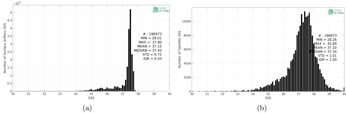
Figure 2: Histograms of SSS from Surface drifters (a) and SMOS-L3-CATDS-CPDC-V321-L2Q (b) considering all match-up pairs per bins of 0.1 over the North Atlantic Ocean Pi-MEP region and for the full satellite product period.
