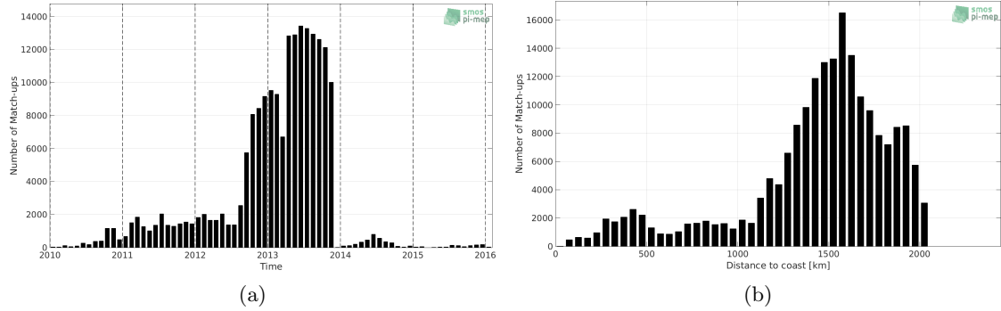
Figure 1: Number of match-ups between Surface drifters and SMOS-L3-CATDS-CPDC-V321-L2Q SSS as a function of time (a) and as function of the distance to coast (b) over the North Atlantic Ocean Pi-MEP region and for the full satellite product period.
