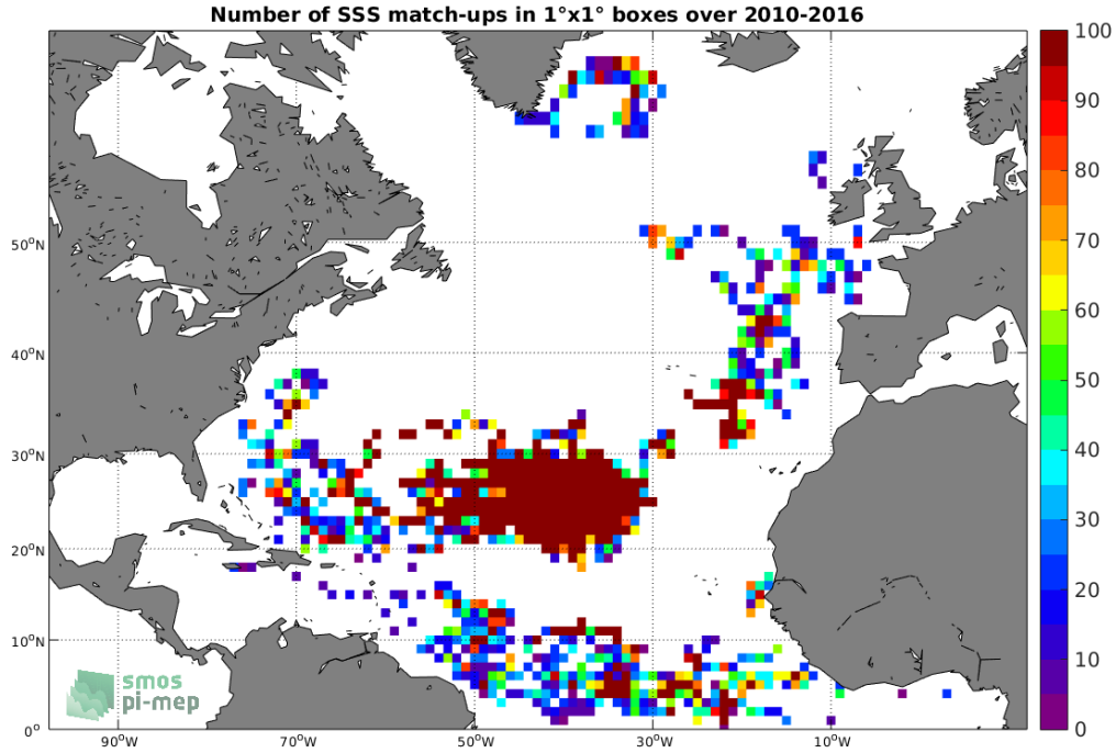
Figure 3: Number of SSS match-ups between Surface drifters SSS and the SMOS-L3-CATDS-CPDC-V321-L2Q SSS product for the North Atlantic Ocean Pi-MEP region over 1^\circ \times 1^\circ boxes and for the full satellite product period.
