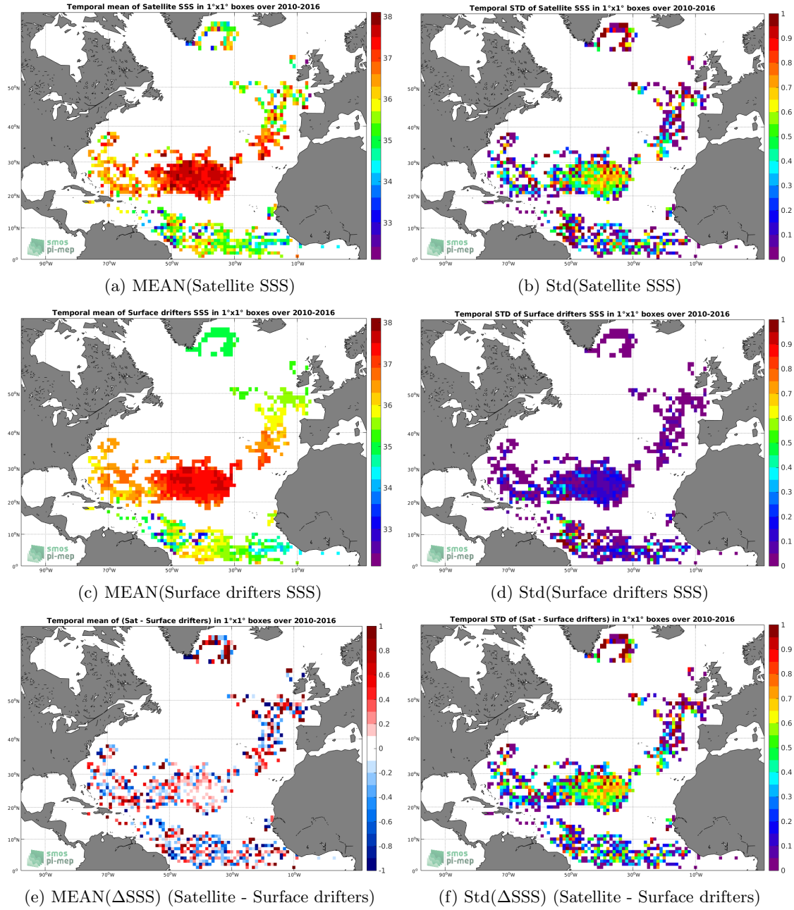
Figure 5: Temporal mean (left) and Std (right) of SSS from SMOS-L3-CATDS-CPDC-V321-L2Q (top), Surface drifters (middle), and of \Delta SSS (Satellite - Surface drifters). Only match-up pairs are used to generate these maps.
