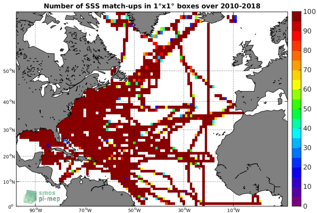
Figure 4: Number of SSS match-ups between TSG-SAMOS SSS and the SMOS-L3-CATDS-CPDC-V317-MONTHLY-25KM SSS product for the North Atlantic Ocean Pi-MEP region over 1^\circ \times 1^\circ boxes and for the full satellite product period.
