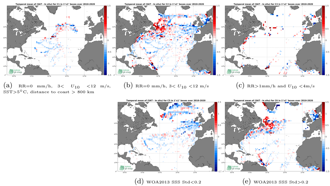
Figure 12: Temporal mean gridded over spatial boxes of size 1^\circ \times 1^\circ of \Delta\text{SSS} (SMOS SSS L3 v317 - Monthly - 25 km (CATDS-CPDC) - TSG (LEGOS-DM)) for 5 different subdatasets corresponding to:RR=0 mm/h, 3 < U_{10} < 12 m/s, SST >5^\circ\text{C} , distance to coast > 800 km (a), RR=0 mm/h, 3 < U_{10} < 12 m/s (b), RR >1 mm/h and U_{10} < 4 m/s (c), WOA2013 SSS Std <0.2 (d), WOA2013 SSS Std >0.2 (e).
