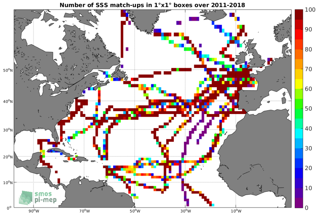
Figure 4: Number of SSS match-ups between TSG (GOSUD-Sailing-ship) SSS and the SMOS SSS L3 v317 - Monthly - 25 km (CATDS-CPDC) SSS product for the North Atlantic Ocean Pi-MEP region over 1°x1° boxes and for the full satellite product period.
