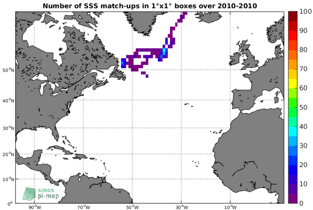
Figure 4: Number of SSS match-ups between Sea mammals SSS and the SMOS-L3-CATDS-CPDC-V317-MONTHLY-25KM SSS product for the North Atlantic Ocean Pi-MEP region over 1^\circ \times 1^\circ boxes and for the full satellite product period.
