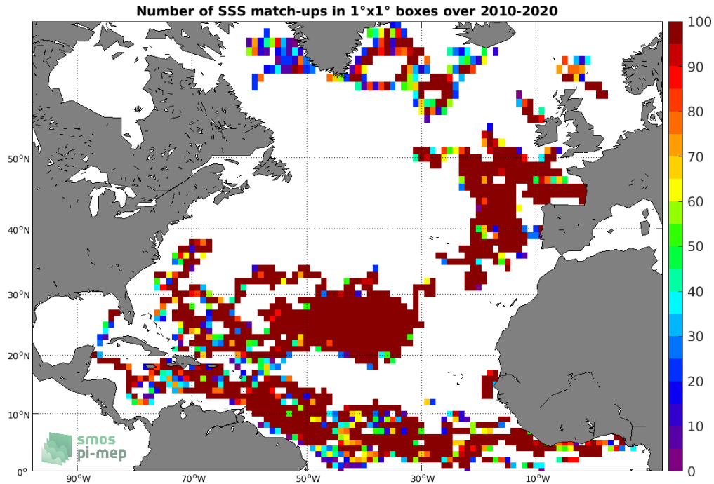
Figure 3: Number of SSS match-ups between Surface drifters SSS and the SMOS SSS L3 v317 - Monthly - 25 km (CATDS-CPDC) SSS product for the North Atlantic Ocean Pi-MEP region over 1^\circ \times 1^\circ boxes and for the full satellite product period.
