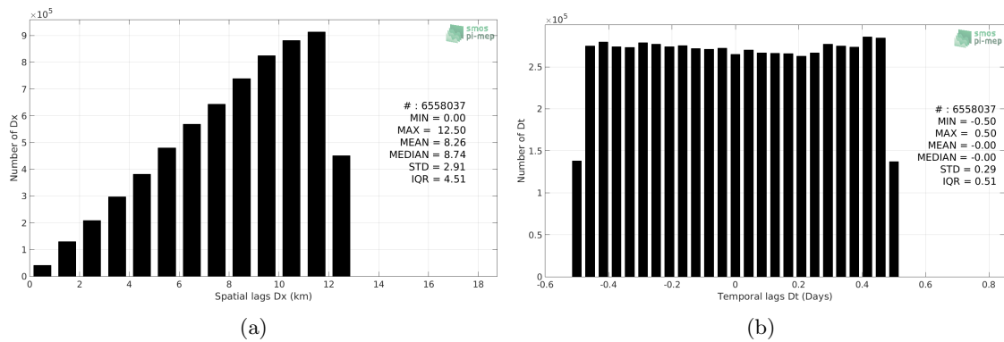
Figure 5: Histograms of the spatial (a) and temporal (b) lags between the location/time of the TSG (SAMOS) measurement and the date of the corresponding SMOS SSS L3 v317 - 10 Days - 25 km (CATDS-CPDC) SSS pixel.
