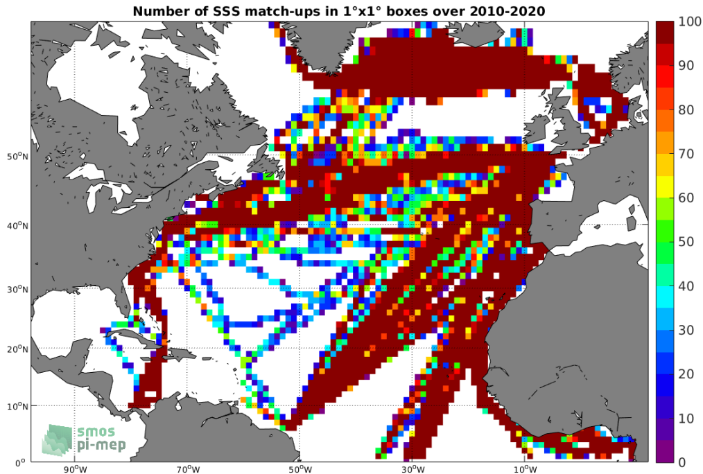
Figure 4: Number of SSS match-ups between TSG (LEGOS-DM) SSS and the SMOS SSS L3 v317 - 10 Days - 25 km (CATDS-CPDC) SSS product for the North Atlantic Ocean Pi-MEP region over 1°x1° boxes and for the full satellite product period.
