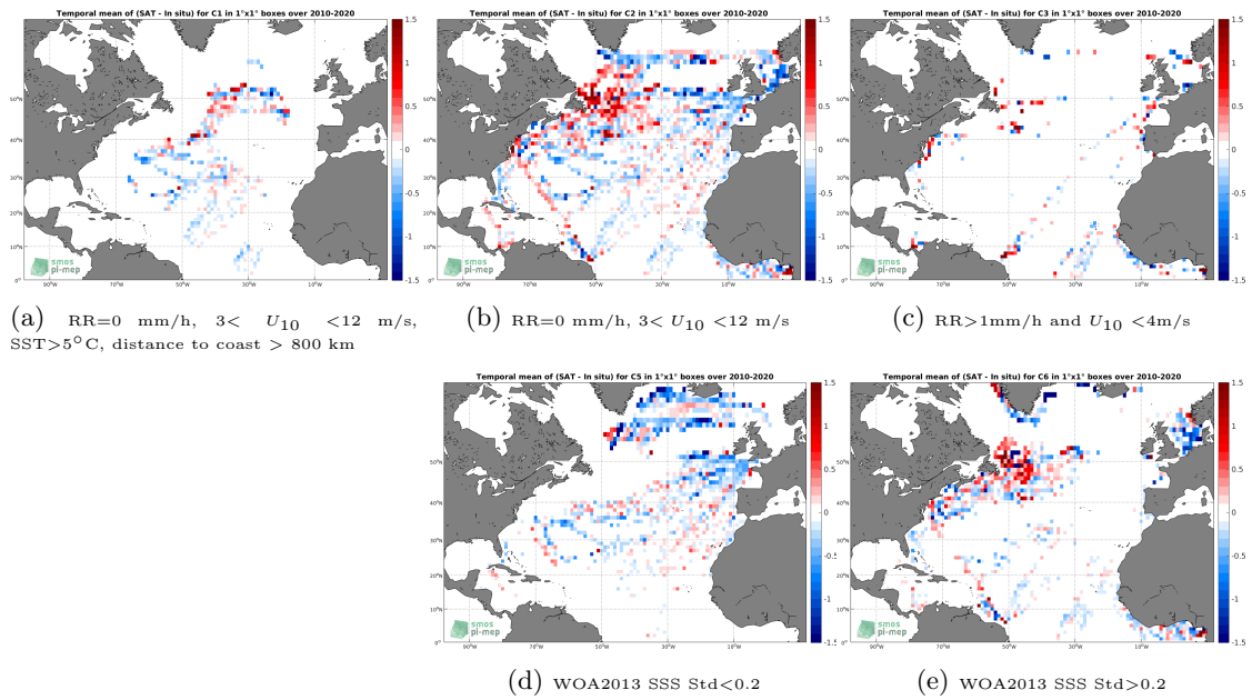
Figure 12: Temporal mean gridded over spatial boxes of size 1°x1° of \Delta SSS (SMOS SSS L3 v317 - 10 Days - 25 km (CATDS-CPDC) - TSG (LEGOS-DM)) for 5 different subdatasets corresponding to:RR=0 mm/h, 3 < U_{10} < 12 m/s, SST>5°C, distance to coast > 800 km (a), RR=0 mm/h, 3 < U_{10} < 12 m/s (b), RR>1mm/h and U_{10} < 4 m/s (c), WOA2013 SSS Std<0.2 (d), WOA2013 SSS Std>0.2 (e).
