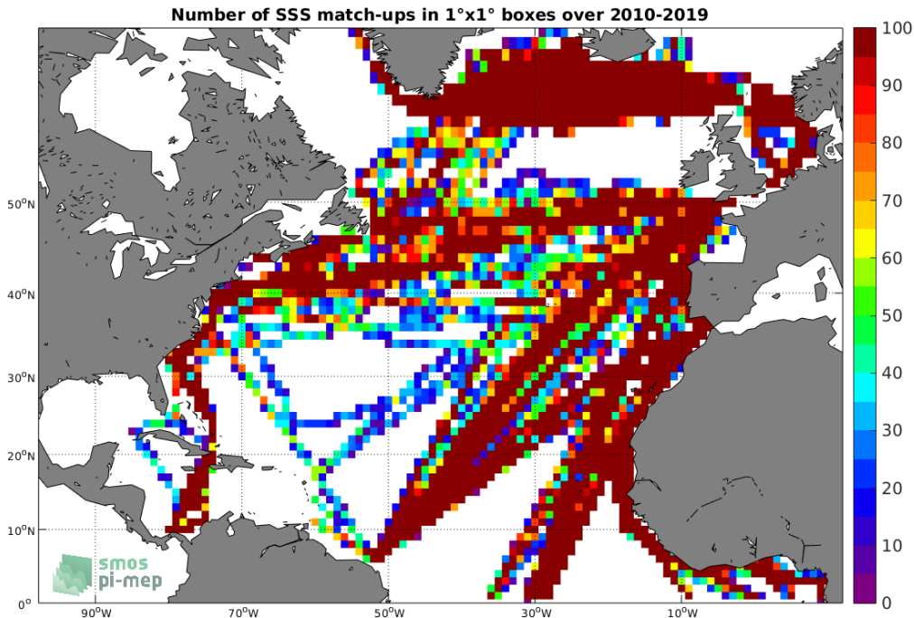
Figure 4: Number of SSS match-ups between TSG-LEGOS-DM SSS and the SMOS L3 v317 - 10 Days - 25 km (CATDS-CPDC) SSS product for the North Atlantic Ocean Pi-MEP region over 1^\circ \times 1^\circ boxes and for the full satellite product period.
