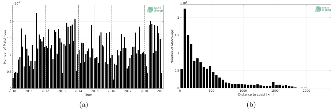
Figure 1: Number of match-ups between TSG-LEGOS-DM and SMOS L3 v317 - 10 Days - 25 km (CATDS-CPDC) SSS as a function of time (a) and as function of the distance to coast (b) over the North Atlantic Ocean Pi-MEP region and for the full satellite product period.
