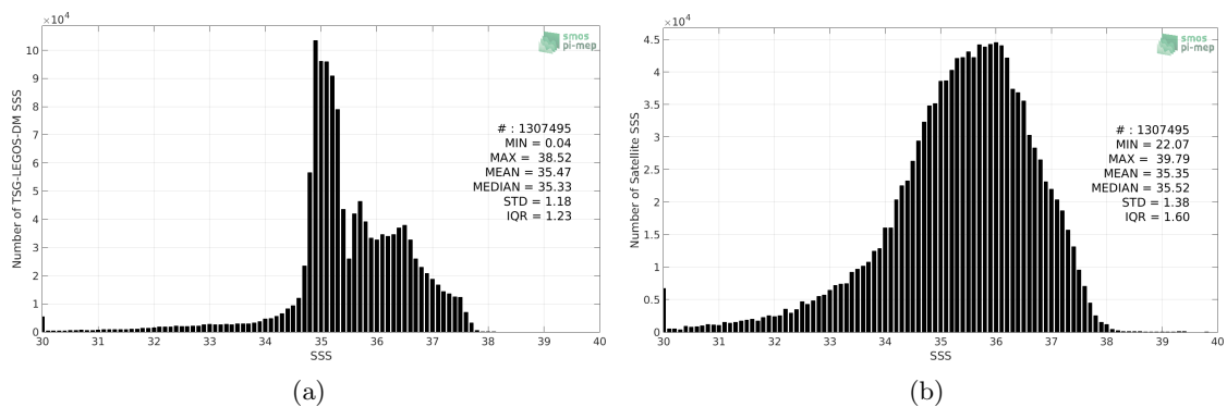
Figure 2: Histograms of SSS from TSG-LEGOS-DM (a) and SMOS L3 v317 - 10 Days - 25 km (CATDS-CPDC) (b) considering all match-up pairs per bins of 0.1 over the North Atlantic Ocean Pi-MEP region and for the full satellite product period.
