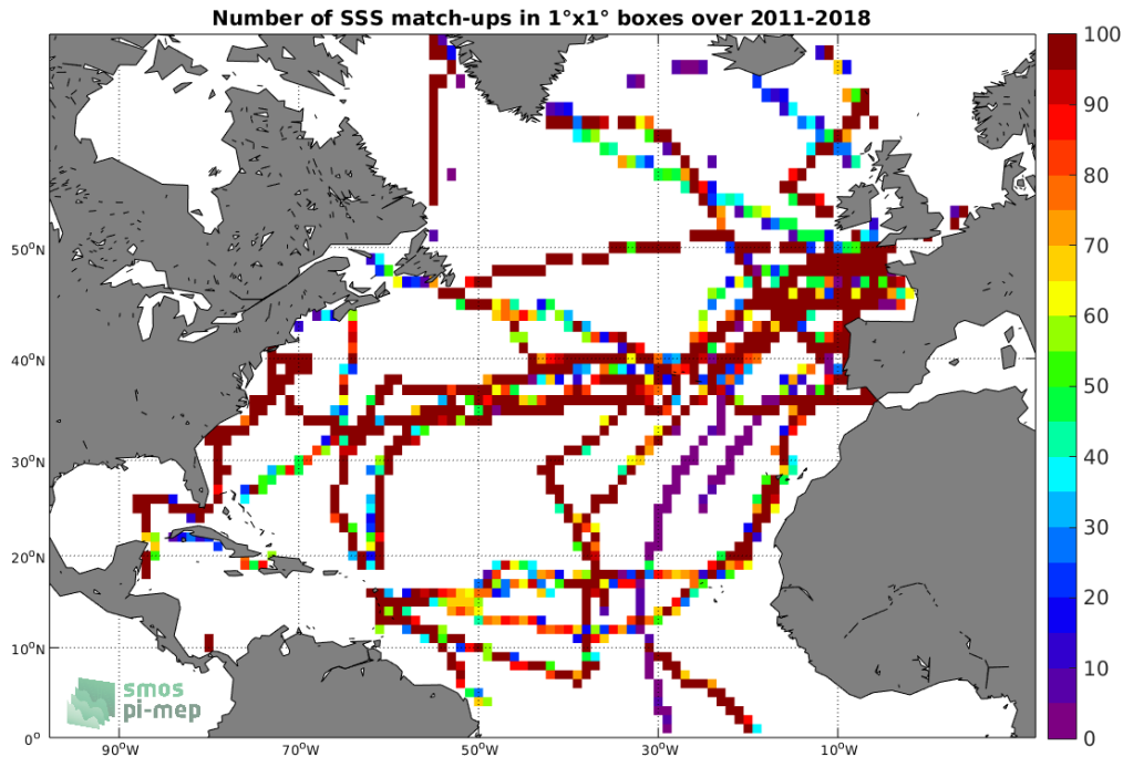
Figure 4: Number of SSS match-ups between TSG (GOSUD-Sailing-ship) SSS and the SMOS SSS L3 v317 - 10 Days - 25 km (CATDS-CPDC) SSS product for the North Atlantic Ocean Pi-MEP region over 1°x1° boxes and for the full satellite product period.
