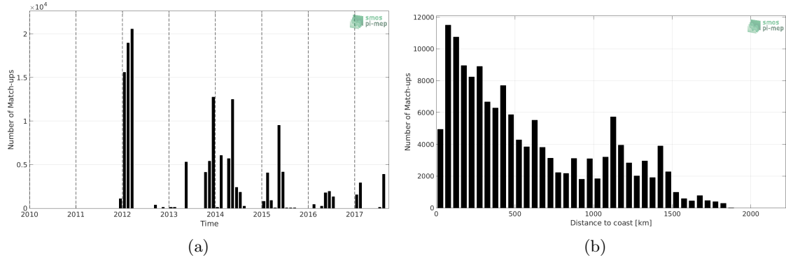
Figure 1: Number of match-ups between TSG-GOSUD-Sailing-ship and SMOS L3 v317 - 10 Days - 25 km (CATDS-CPDC) SSS as a function of time (a) and as function of the distance to coast (b) over the North Atlantic Ocean Pi-MEP region and for the full satellite product period.
