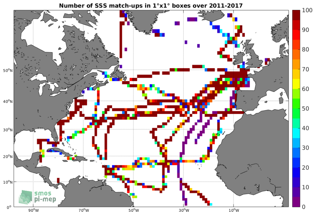
Figure 4: Number of SSS match-ups between TSG-GOSUD-Sailing-ship SSS and the SMOS L3 v317 - 10 Days - 25 km (CATDS-CPDC) SSS product for the North Atlantic Ocean Pi-MEP region over 1°x1° boxes and for the full satellite product period.
