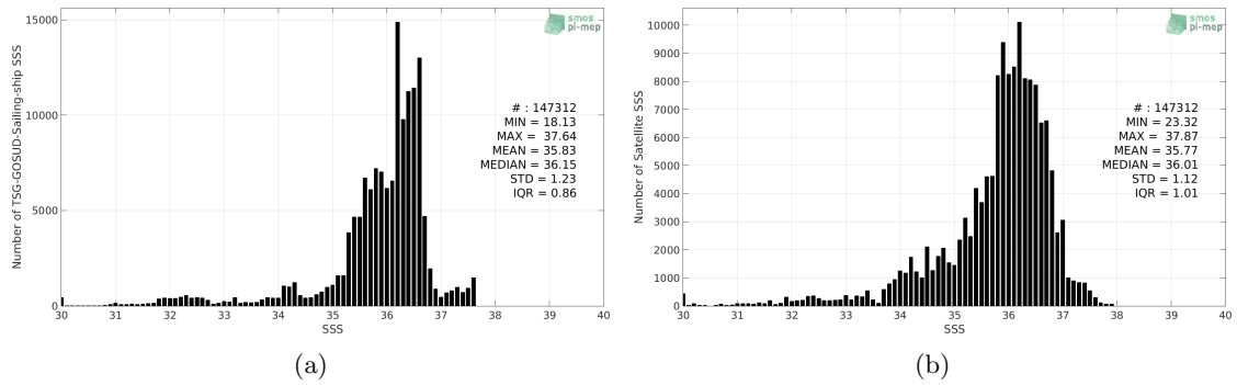
Figure 2: Histograms of SSS from TSG-GOSUD-Sailing-ship (a) and SMOS L3 v317 - 10 Days - 25 km (CATDS-CPDC) (b) considering all match-up pairs per bins of 0.1 over the North Atlantic Ocean Pi-MEP region and for the full satellite product period.
