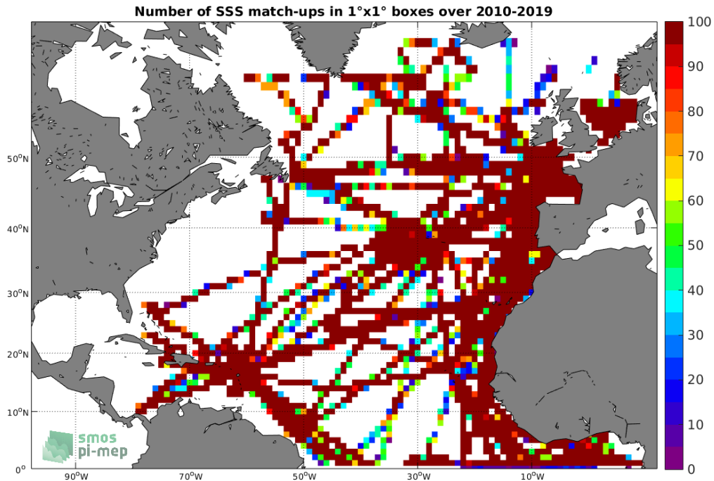
Figure 4: Number of SSS match-ups between TSG (GOSUD-Research-vessel) SSS and the SMOS SSS L3 v317 - 10 Days - 25 km (CATDS-CPDC) SSS product for the North Atlantic Ocean Pi-MEP region over 1°x1° boxes and for the full satellite product period.
