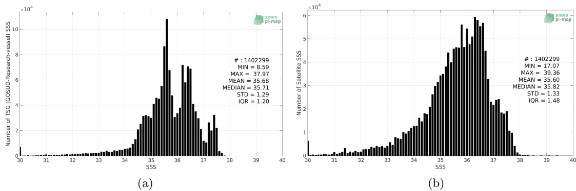
Figure 2: Histograms of SSS from TSG (GOSUD-Research-vessel) (a) and SMOS SSS L3 v317 - 10 Days - 25 km (CATDS-CPDC) (b) considering all match-up pairs per bins of 0.1 over the North Atlantic Ocean Pi-MEP region and for the full satellite product period.
