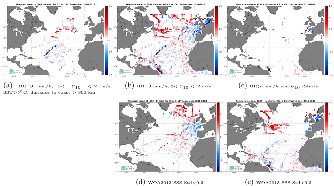
Figure 12: Temporal mean gridded over spatial boxes of size 1^\circ \times 1^\circ of \Delta\text{SSS} (SMOS SSS L3 v317 - 10 Days - 25 km (CATDS-CPDC) - TSG (GOSUD-Research-vessel)) for 5 different subdatasets corresponding to: RR=0 mm/h, 3 < U_{10} < 12 m/s, SST > 5°C, distance to coast > 800 km (a), RR=0 mm/h, 3 < U_{10} < 12 m/s (b), RR > 1mm/h and U_{10} < 4 m/s (c), WOA2013 SSS Std < 0.2 (d), WOA2013 SSS Std > 0.2 (e).
