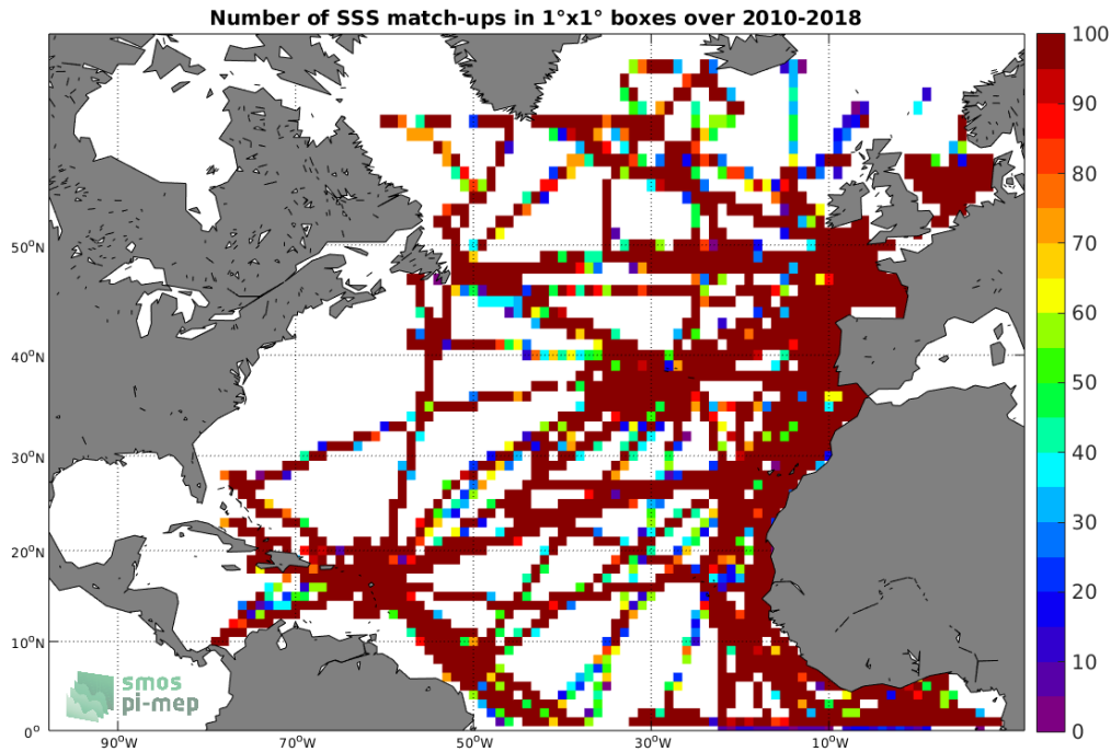
Figure 4: Number of SSS match-ups between TSG (GOSUD-Research-vessel) SSS and the SMOS SSS L3 v317 - 10 Days - 25 km (CATDS-CPDC) SSS product for the North Atlantic Ocean Pi-MEP region over 1^\circ \times 1^\circ boxes and for the full satellite product period.
