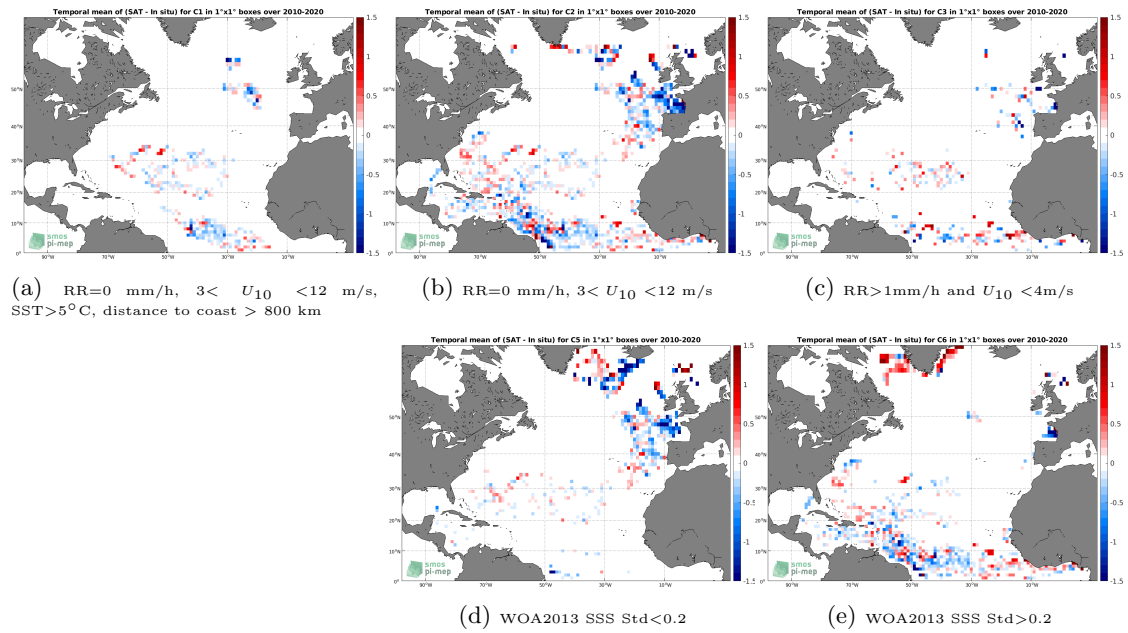
Figure 11: Temporal mean gridded over spatial boxes of size 1^\circ \times 1^\circ of \Delta\text{SSS} (SMOS SSS L3 v317 - 10 Days - 25 km (CATDS-CPDC) - Surface drifters) for 5 different subdatasets corresponding to:RR=0 mm/h, 3 < U_{10} < 12 m/s, SST >5^\circ\text{C} , distance to coast > 800 km (a), RR=0 mm/h, 3 < U_{10} < 12 m/s (b), RR >1 mm/h and U_{10} < 4 m/s (c), WOA2013 SSS Std <0.2 (d), WOA2013 SSS Std >0.2 (e).
