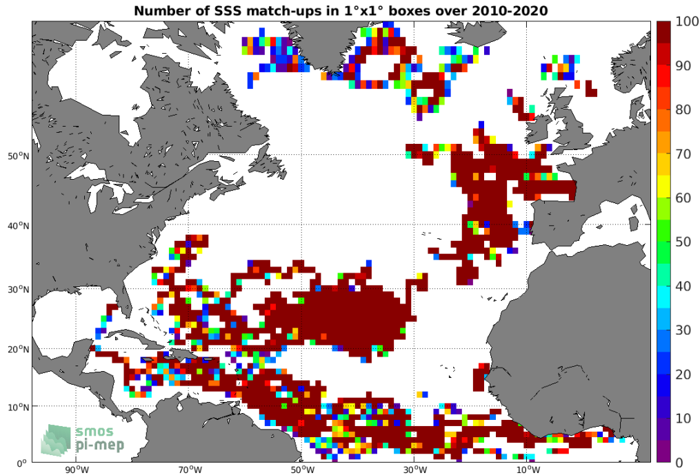
Figure 3: Number of SSS match-ups between Surface drifters SSS and the SMOS SSS L3 v317 - 10 Days - 25 km (CATDS-CPDC) SSS product for the North Atlantic Ocean Pi-MEP region over 1^\circ \times 1^\circ boxes and for the full satellite product period.
