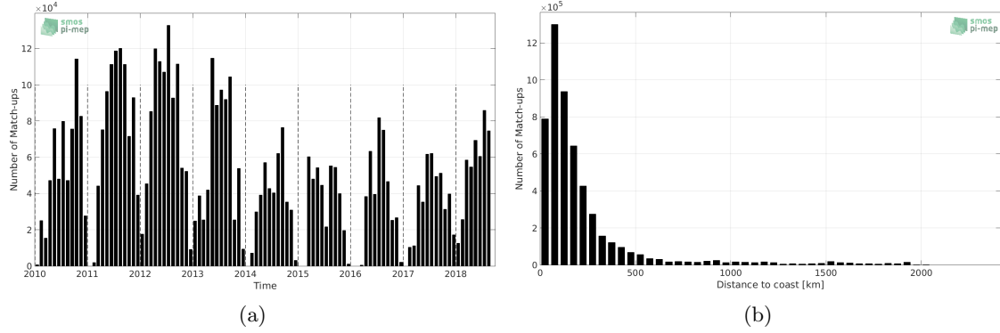
Figure 1: Number of match-ups between TSG-SAMOS and SMOS-L3-CATDS-CPDC-V3-MONTHLY-25KM SSS as a function of time (a) and as function of the distance to coast (b) over the North Atlantic Ocean Pi-MEP region and for the full satellite product period.
