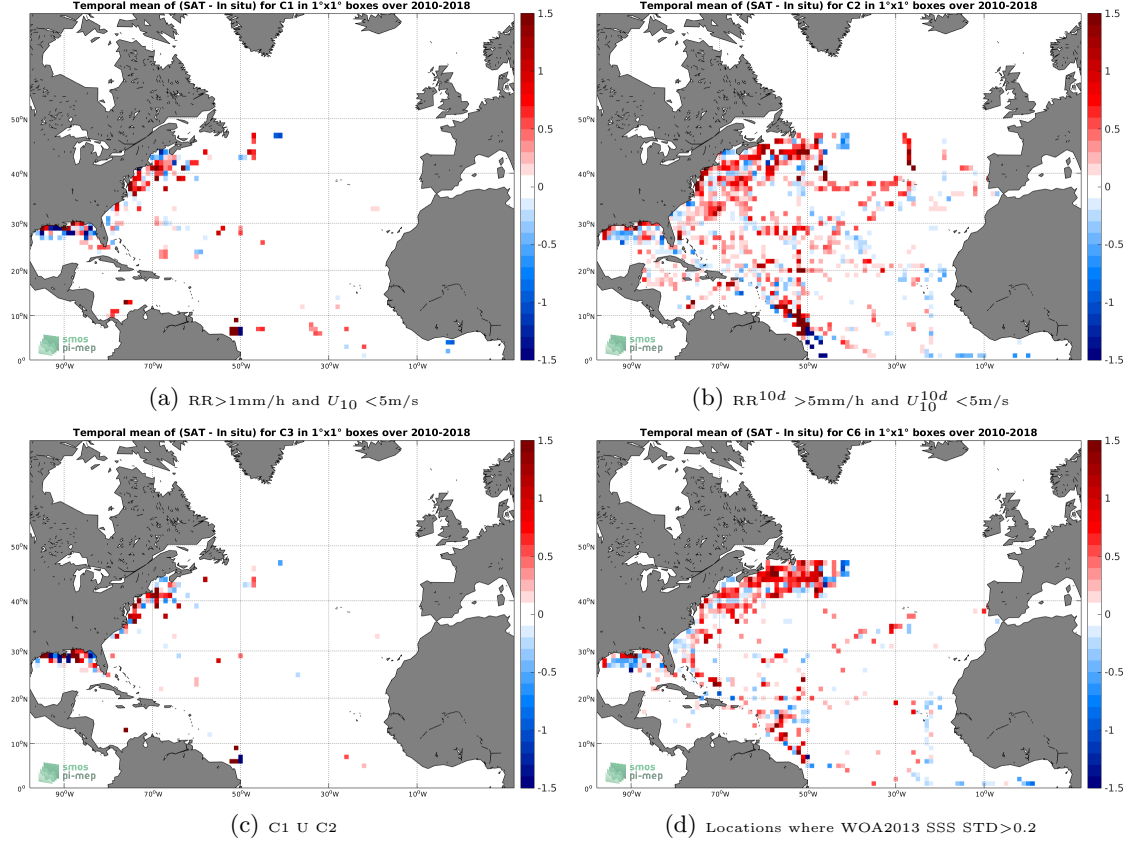
Figure 12: Temporal mean gridded over spatial boxes of size 1^\circ \times 1^\circ of \Delta SSS (SMOS-L3-CATDS-CPDC-V3-MONTHLY-25KM - TSG-SAMOS) for 4 different subdatasets corresponding to: RR > 1\text{mm/h} and U_{10} < 5\text{m/s} (a), RR^{10d} > 5\text{mm/h} and U_{10}^{10d} < 5\text{m/s} (b), C1 U C2 (c), Locations where WOA2013 SSS STD > 0.2 (d).
