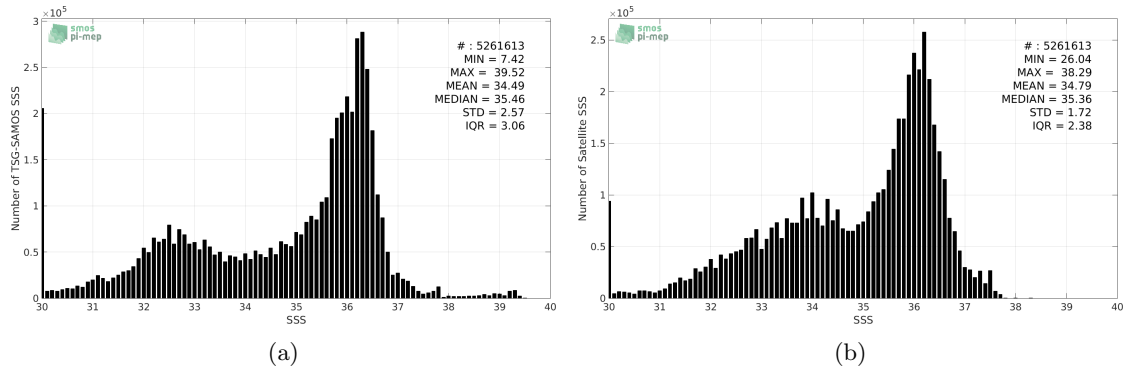
Figure 2: Histograms of SSS from TSG-SAMOS (a) and SMOS-L3-CATDS-CPDC-V3-MONTHLY-25KM (b) considering all match-up pairs per bins of 0.1 over the North Atlantic Ocean Pi-MEP region and for the full satellite product period.
