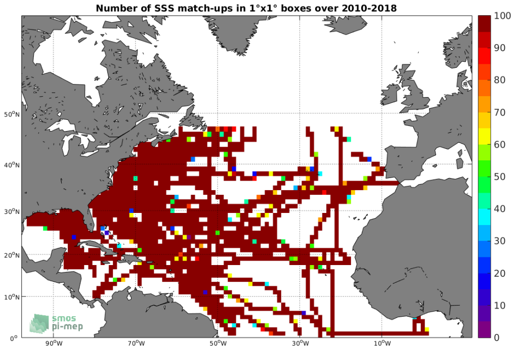
Figure 4: Number of SSS match-ups between TSG-SAMOS SSS and the SMOS-L3-CATDS-CPDC-V3-MONTHLY-25KM SSS product for the North Atlantic Ocean Pi-MEP region over 1^\circ \times 1^\circ boxes and for the full satellite product period.
