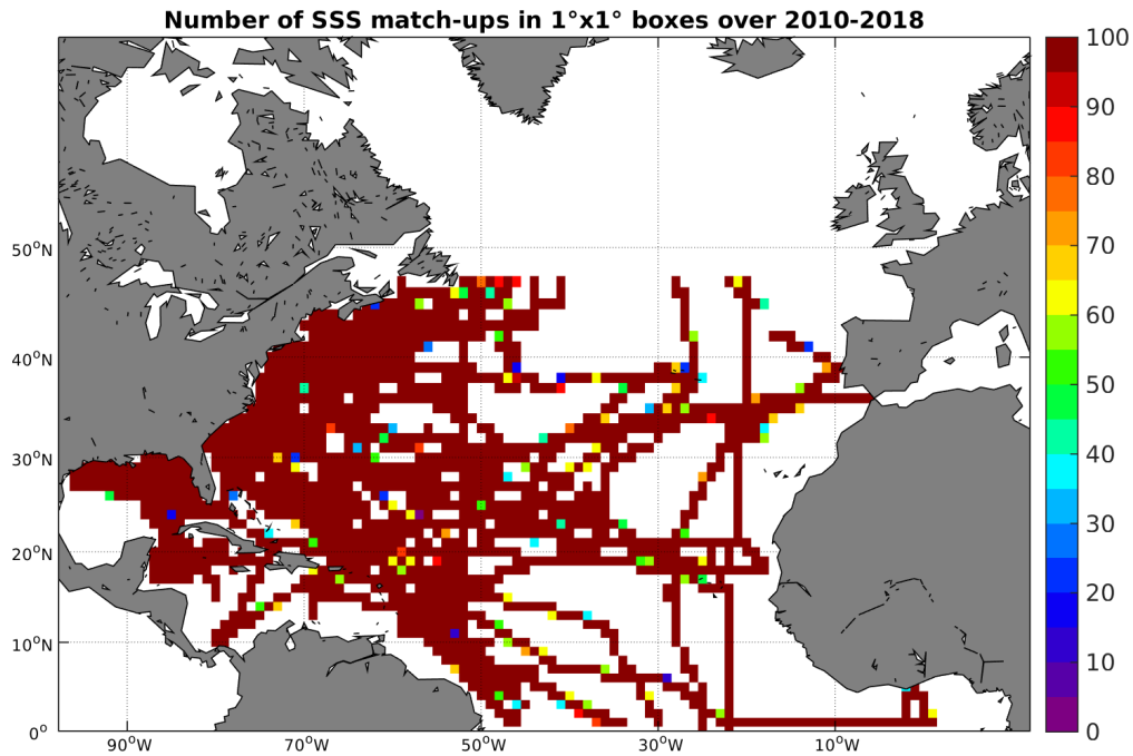
Figure 4: Number of SSS match-ups between TSG-SAMOS SSS and the SMOS-L3-CATDS-CPDC-V3-MONTHLY-25KM SSS product for the North Atlantic Ocean Pi-MEP region over 1°x1° boxes and for the full satellite product period.
