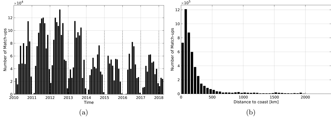
Figure 1: Number of match-ups between TSG-SAMOS and SMOS-L3-CATDS-CPDC-V3-MONTHLY-25KM SSS as a function of time (a) and as function of the distance to coast (b) over the North Atlantic Ocean Pi-MEP region and for the full satellite product period.
