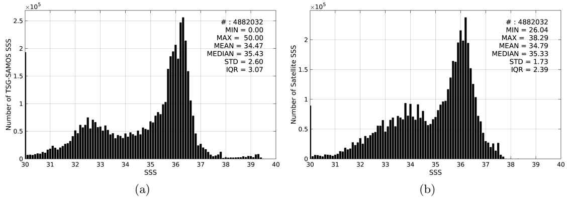
Figure 2: Histograms of SSS from TSG-SAMOS (a) and SMOS-L3-CATDS-CPDC-V3-MONTHLY-25KM (b) considering all match-up pairs per bins of 0.1 over the North Atlantic Ocean Pi-MEP region and for the full satellite product period.
