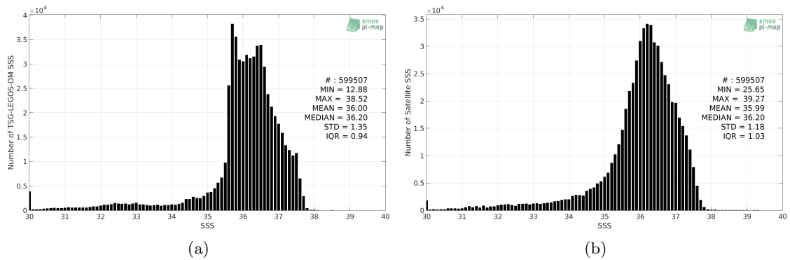
Figure 2: Histograms of SSS from TSG-LEGOS-DM (a) and SMOS-L3-CATDS-CPDC-V3-MONTHLY-25KM (b) considering all match-up pairs per bins of 0.1 over the North Atlantic Ocean Pi-MEP region and for the full satellite product period.
