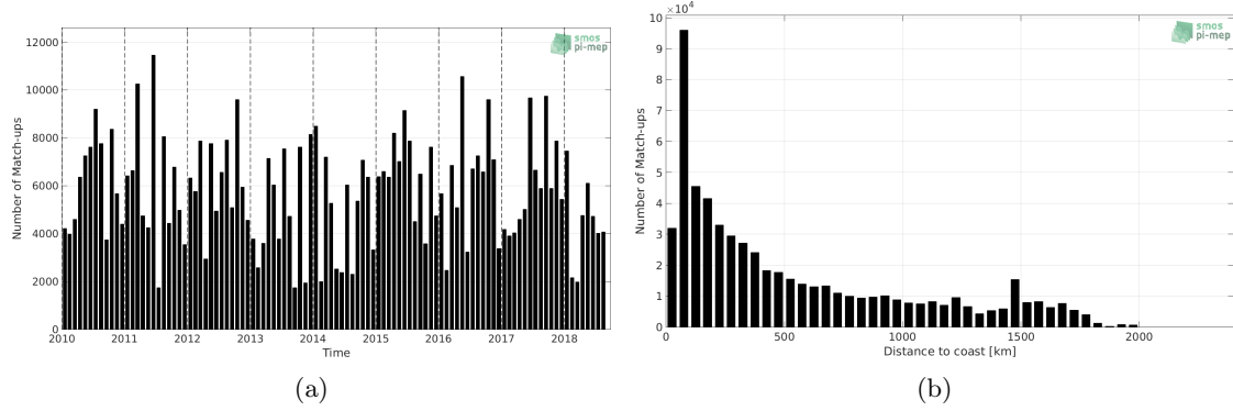
Figure 1: Number of match-ups between TSG-LEGOS-DM and SMOS-L3-CATDS-CPDC-V3-MONTHLY-25KM SSS as a function of time (a) and as function of the distance to coast (b) over the North Atlantic Ocean Pi-MEP region and for the full satellite product period.
