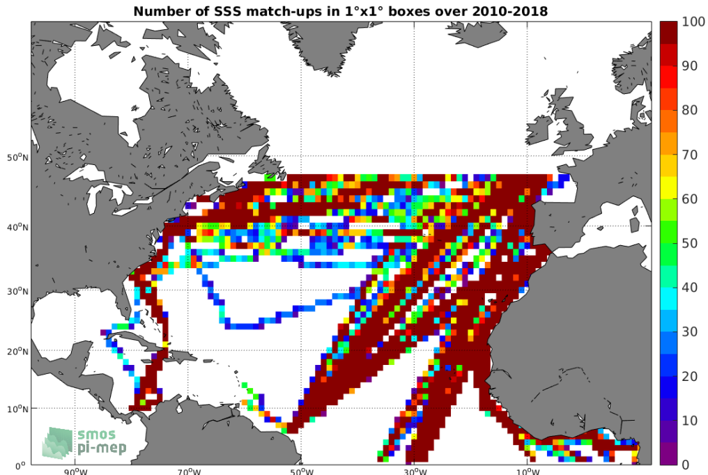
Figure 4: Number of SSS match-ups between TSG-LEGOS-DM SSS and the SMOS-L3-CATDS-CPDC-V3-MONTHLY-25KM SSS product for the North Atlantic Ocean Pi-MEP region over 1^\circ \times 1^\circ boxes and for the full satellite product period.
