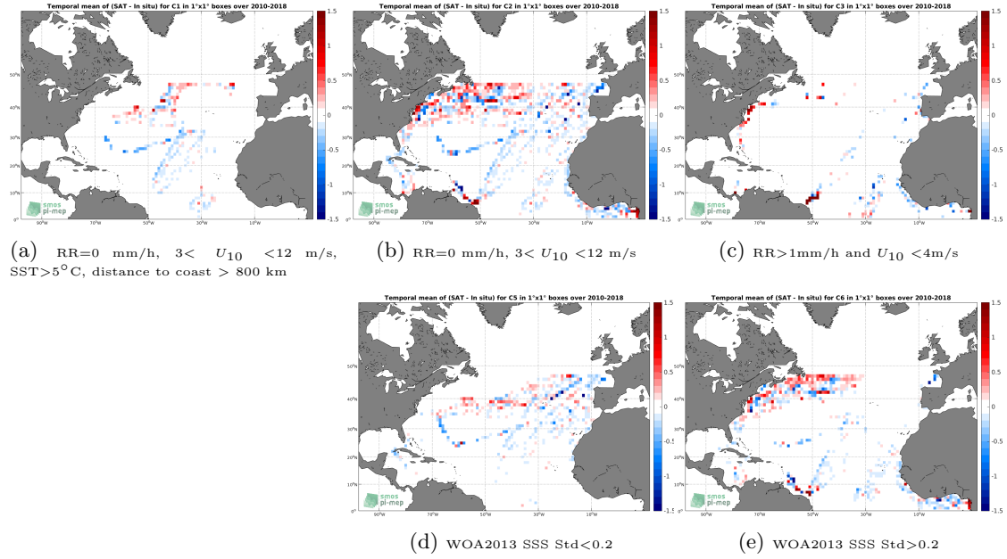
Figure 12: Temporal mean gridded over spatial boxes of size 1^\circ \times 1^\circ of \Delta SSS (SMOS-L3-CATDS-CPDC-V3-MONTHLY-25KM - TSG-LEGOS-DM) for 5 different subdatasets corresponding to: RR=0 mm/h, 3 < U_{10} < 12 m/s, SST >5^\circ\text{C} , distance to coast > 800 km (a), RR=0 mm/h, 3 < U_{10} < 12 m/s (b), RR >1 mm/h and U_{10} < 4 m/s (c), WOA2013 SSS Std <0.2 (d), WOA2013 SSS Std >0.2 (e).
